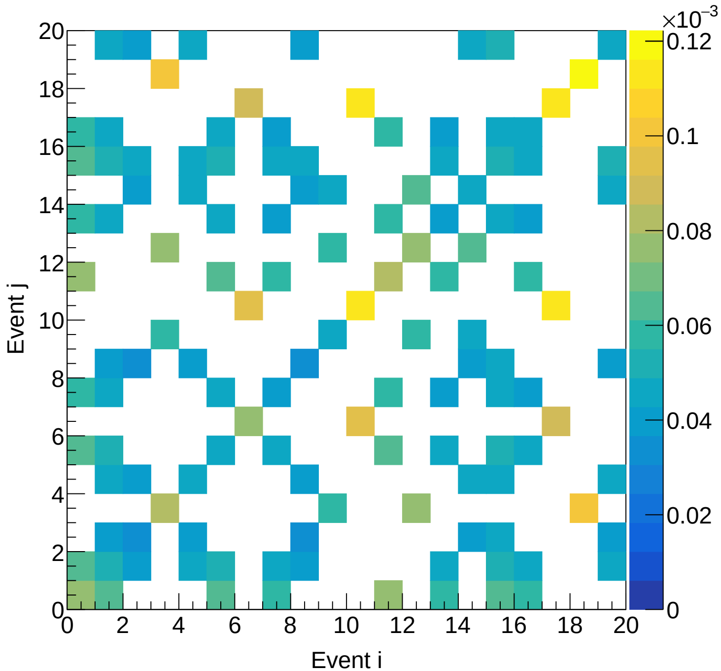
LD2 (mix) Covariance | M: [5.1, 5.4) xF: [0.05, 0.10)
