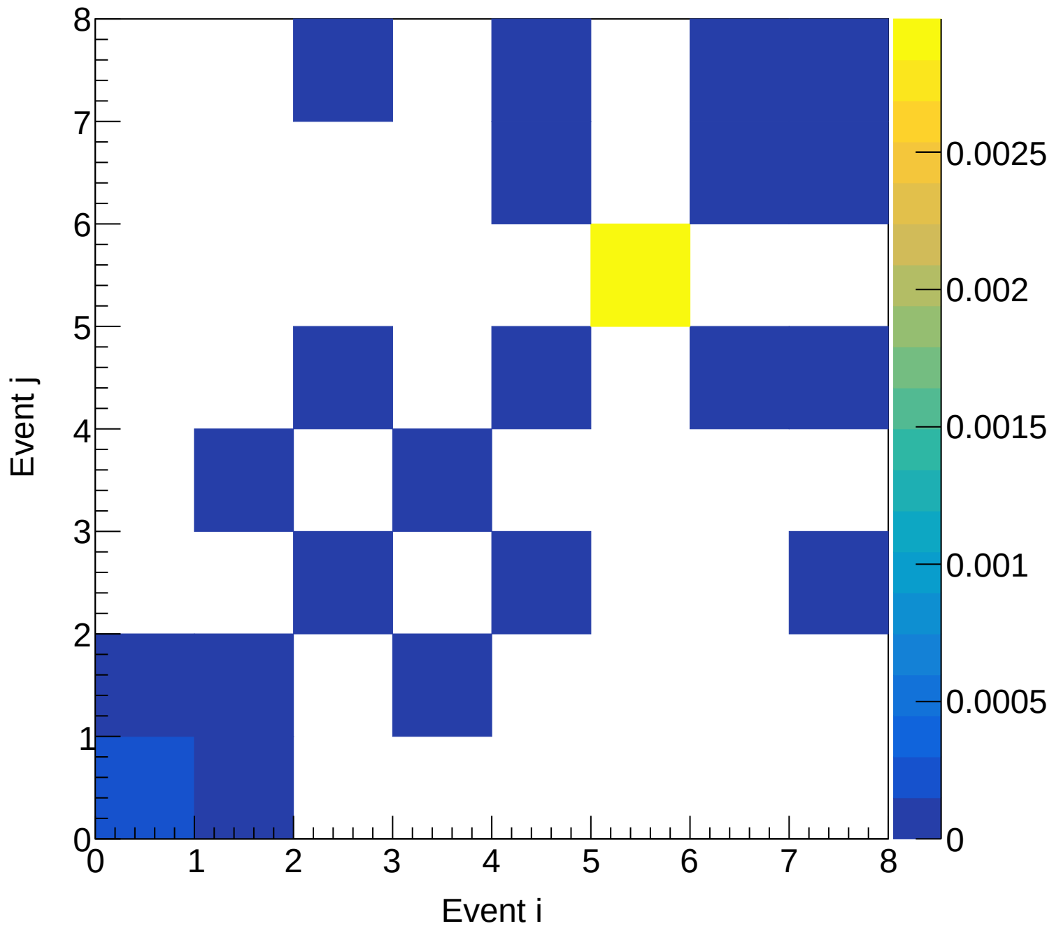
LD2 (mix) Covariance | M: [5.7, 6.0] xF: [0.05, 0.10)
