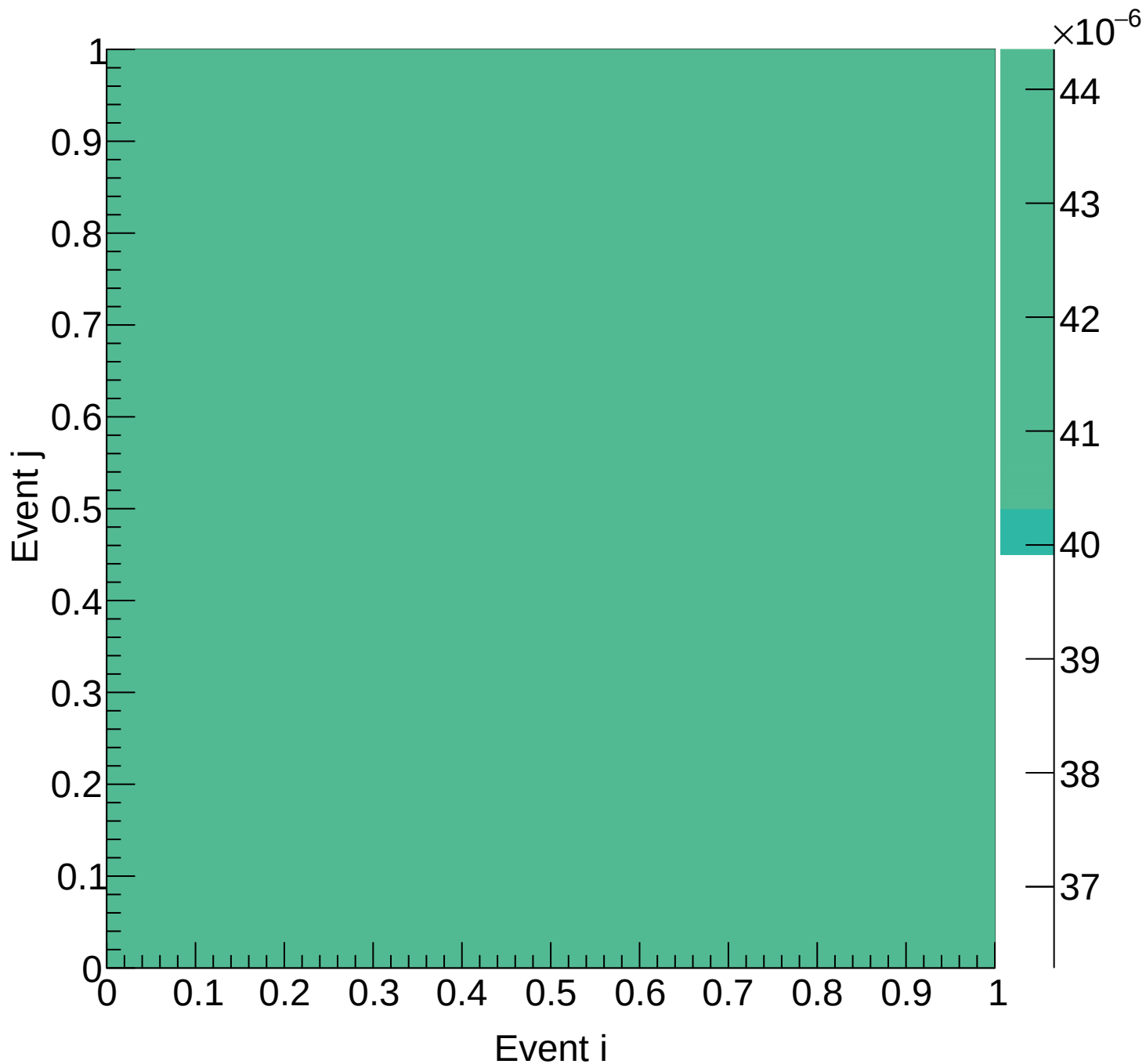
LD2 (mix) Covariance | M: [6.0, 6.3) xF: [0.05, 0.10)
