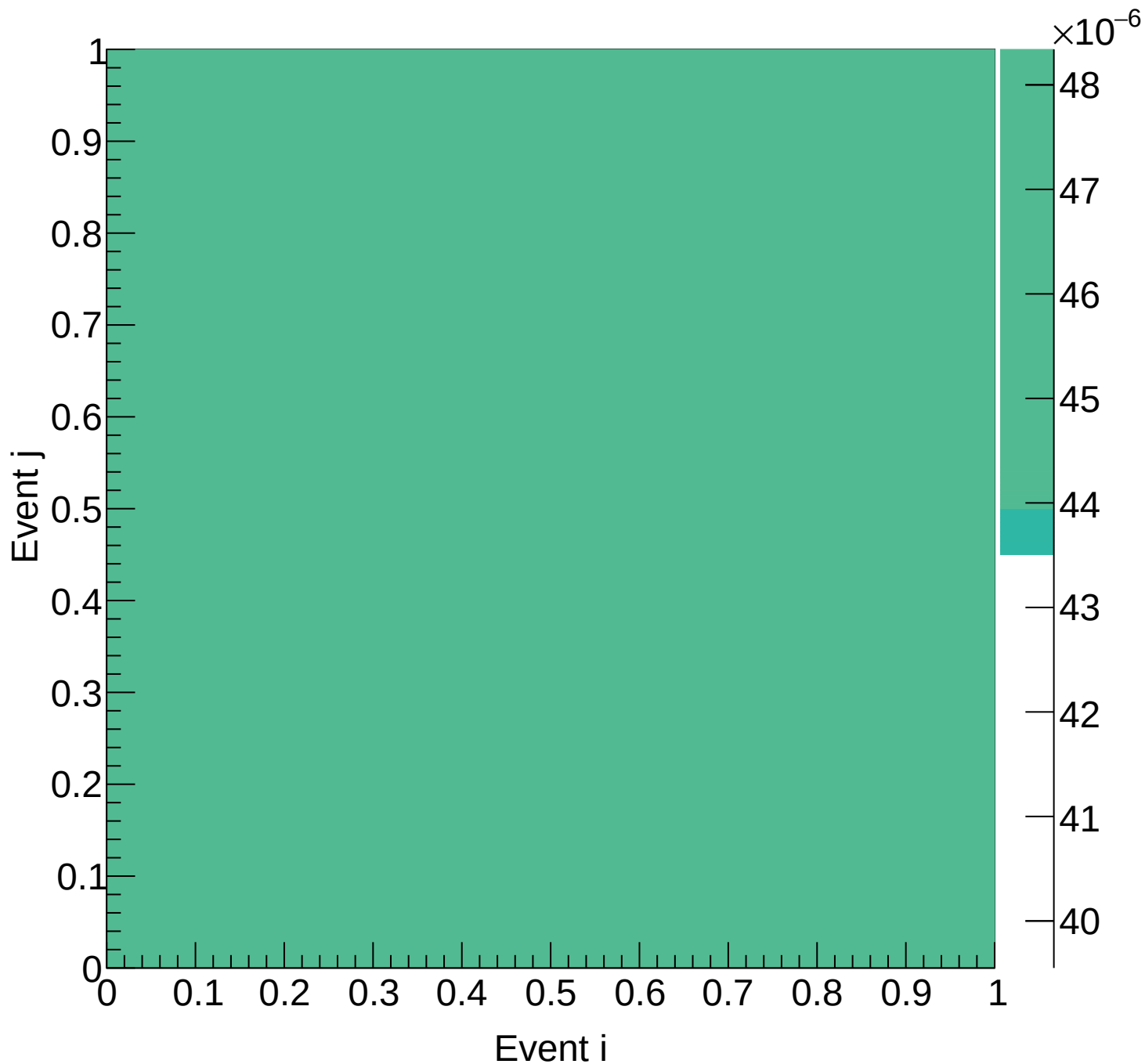
LD2 (mix) Covariance | M: [6.6, 6.9) xF: [0.05, 0.10)
