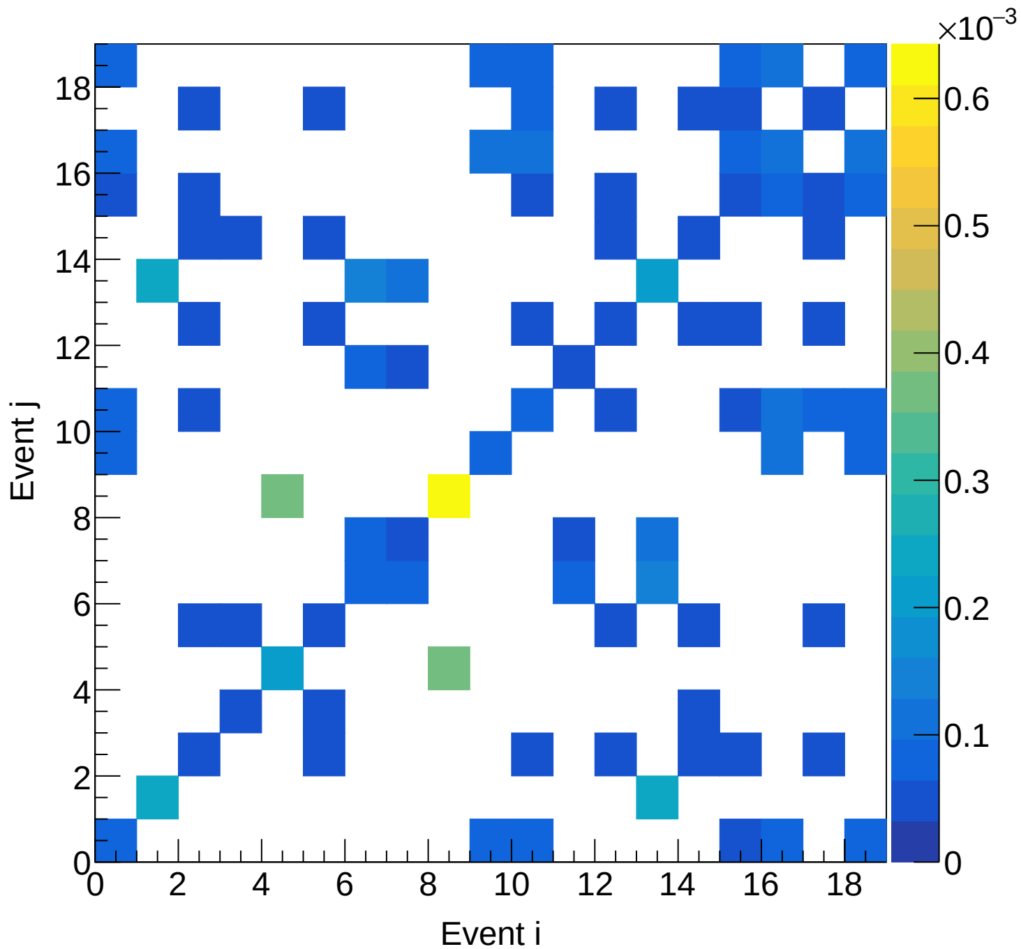
LD2 (mix) Covariance | M: [4.8, 5.1] xF: [0.10, 0.15)
