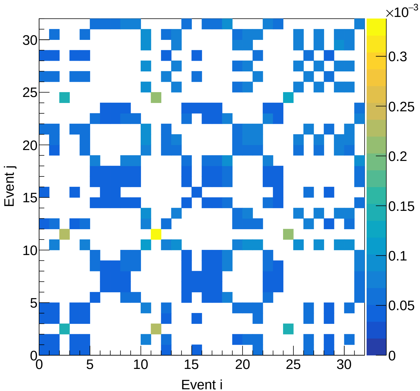
LD2 (mix) Covariance | M: [4.8, 5.1) xF: [0.15, 0.20)
