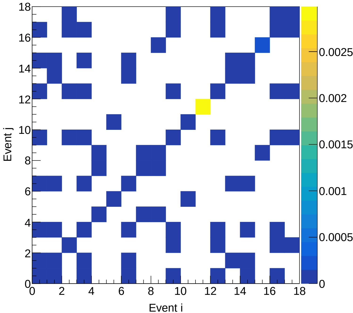
LD2 (mix) Covariance | M: [5.4, 5.7) xF: [0.15, 0.20)
