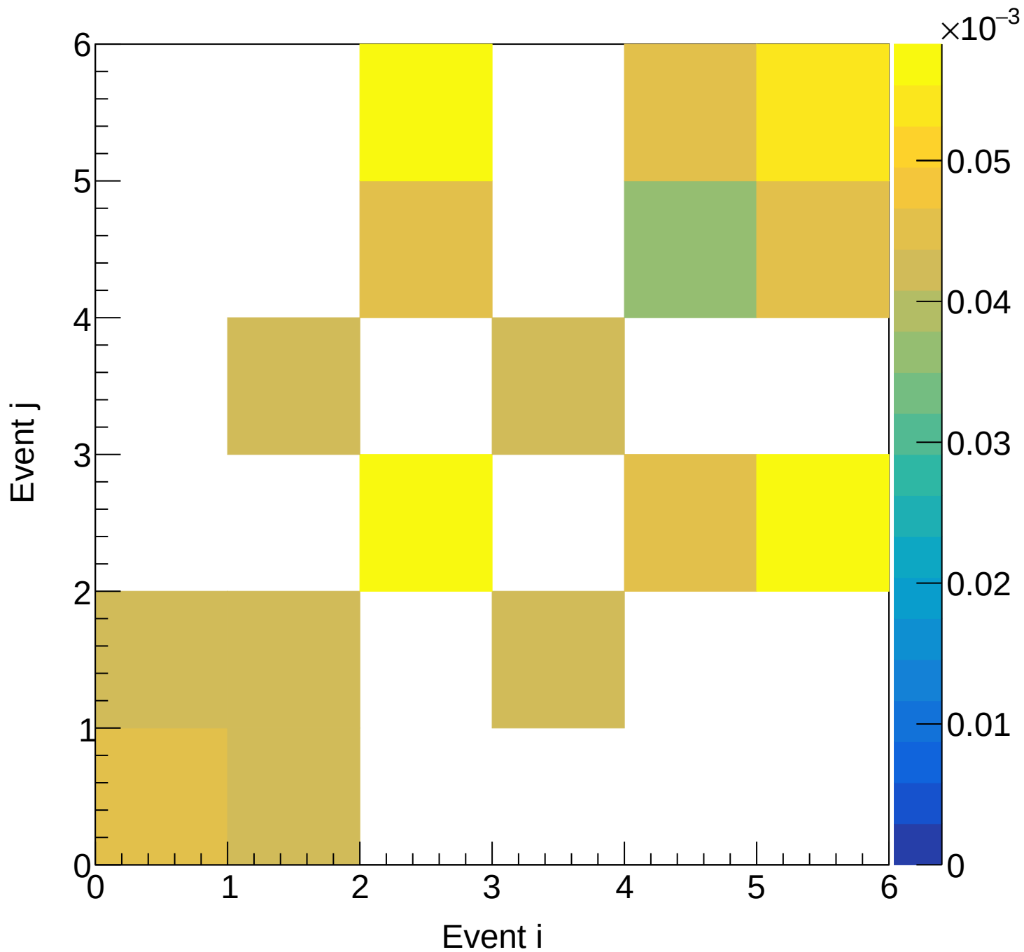
LD2 (mix) Covariance | M: [5.7, 6.0) xF: [0.15, 0.20)
