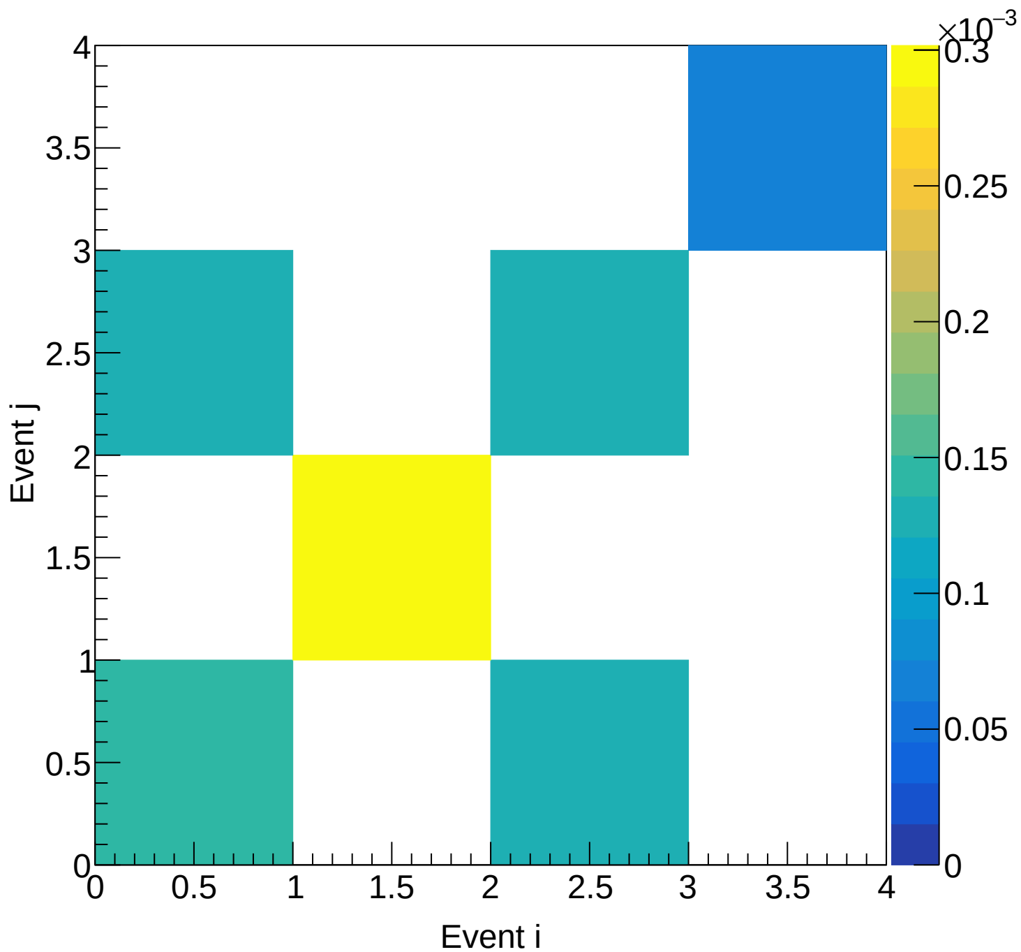
LD2 (mix) Covariance | M: [6.0, 6.3) xF: [0.15, 0.20)
