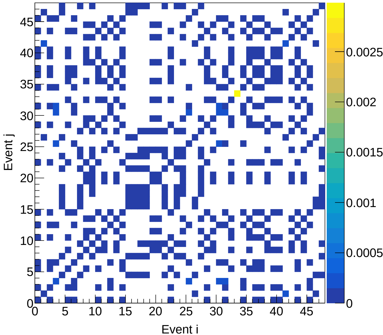
LD2 (mix) Covariance | M: [4.5, 4.8) xF: [0.20, 0.25)
