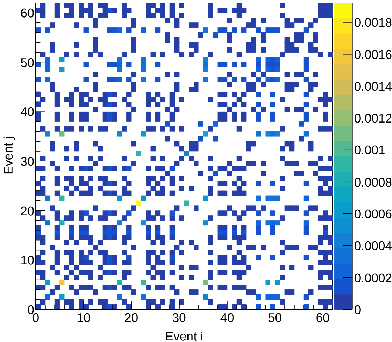
LD2 (mix) Covariance | M: [4.2, 4.5) xF: [0.25, 0.30)
