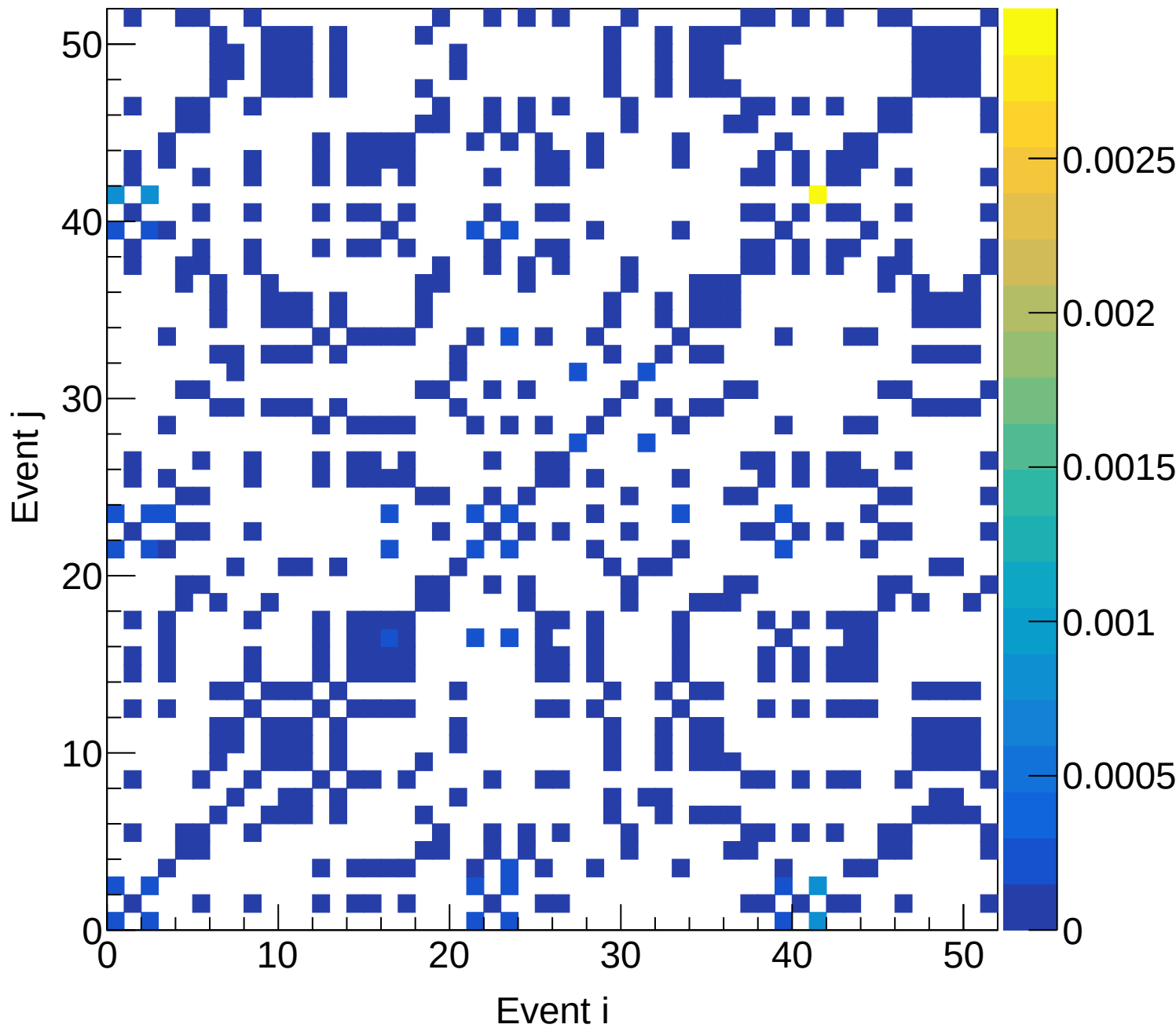
LD2 (mix) Covariance | M: [4.5, 4.8) xF: [0.25, 0.30)
