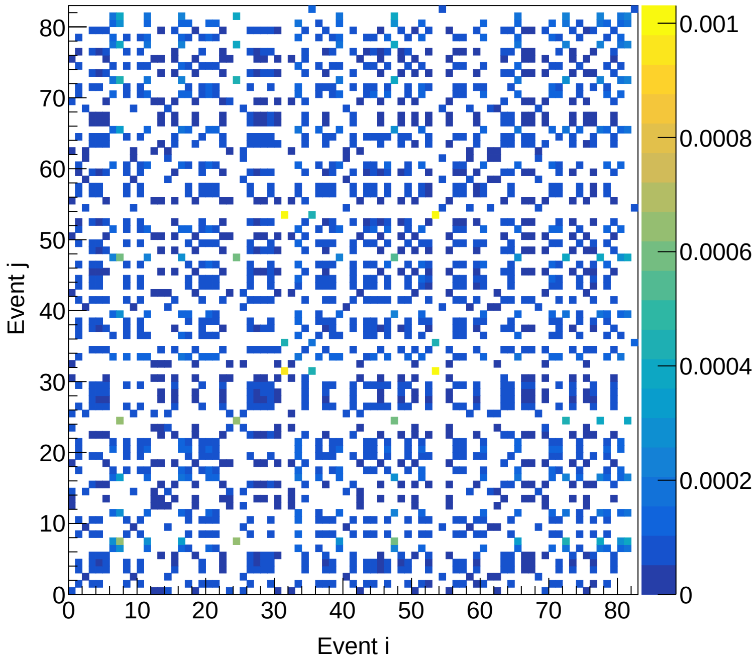
LD2 (mix) Covariance | M: [3.9, 4.2) xF: [0.30, 0.35)
