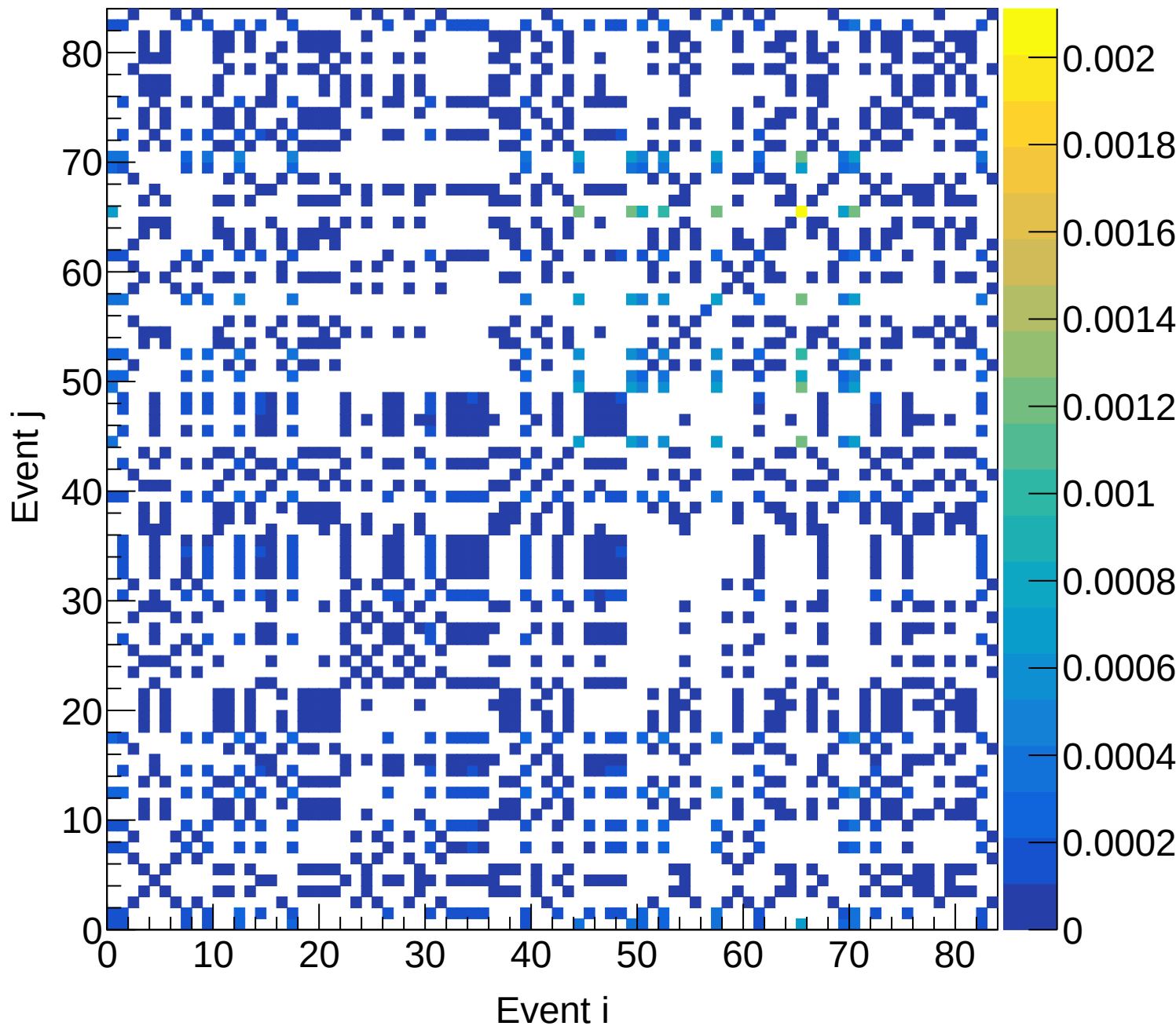
LD2 (mix) Covariance | M: [4.2, 4.5) xF: [0.30, 0.35)
