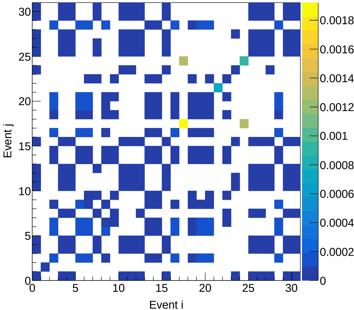
LD2 (mix) Covariance | M: [4.8, 5.1) xF: [0.30, 0.35)
