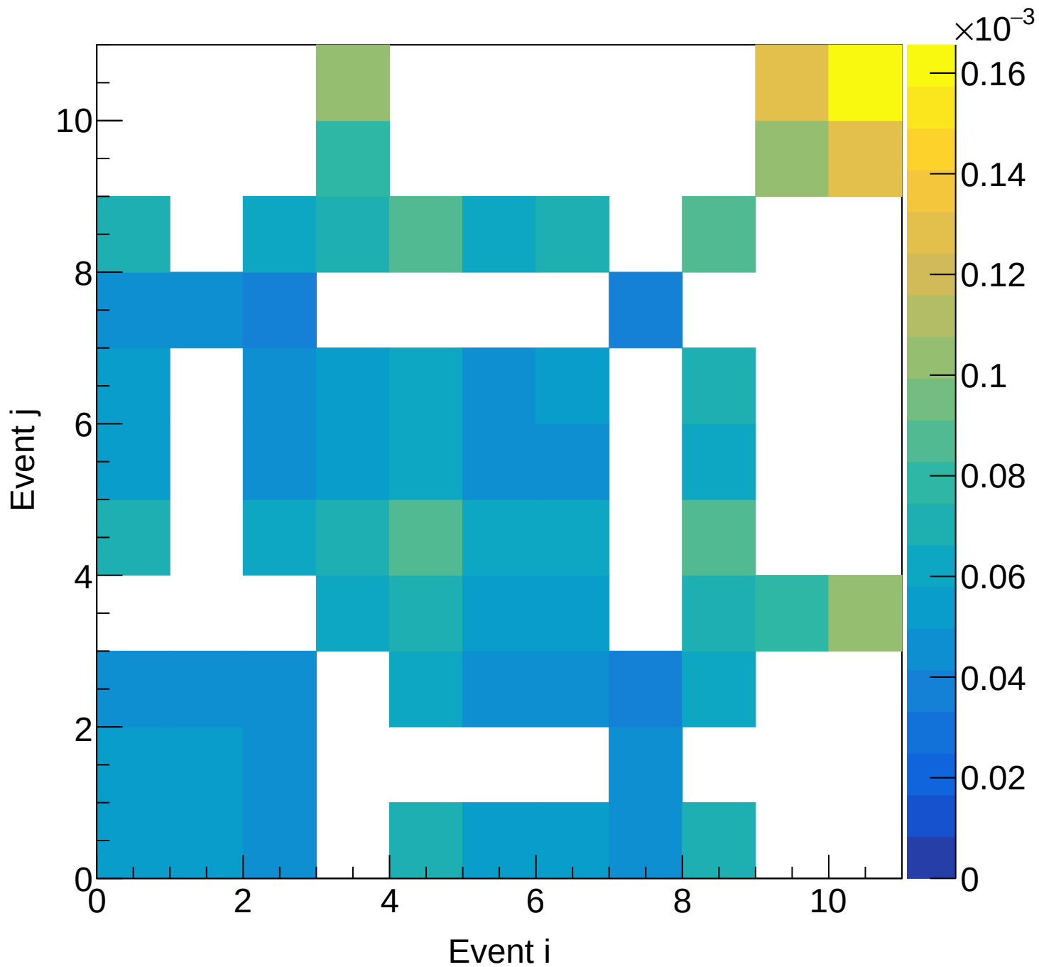
LD2 (mix) Covariance | M: [5.1, 5.4) xF: [0.30, 0.35)
