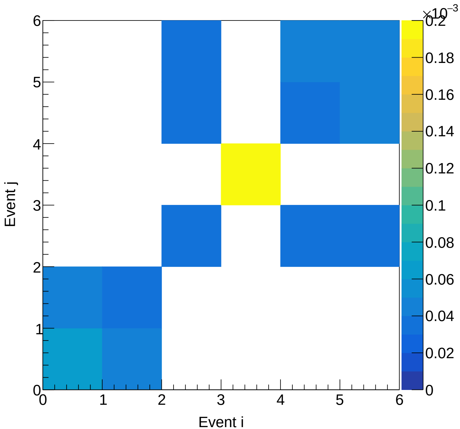
LD2 (mix) Covariance | M: [6.0, 6.3) xF: [0.30, 0.35)
