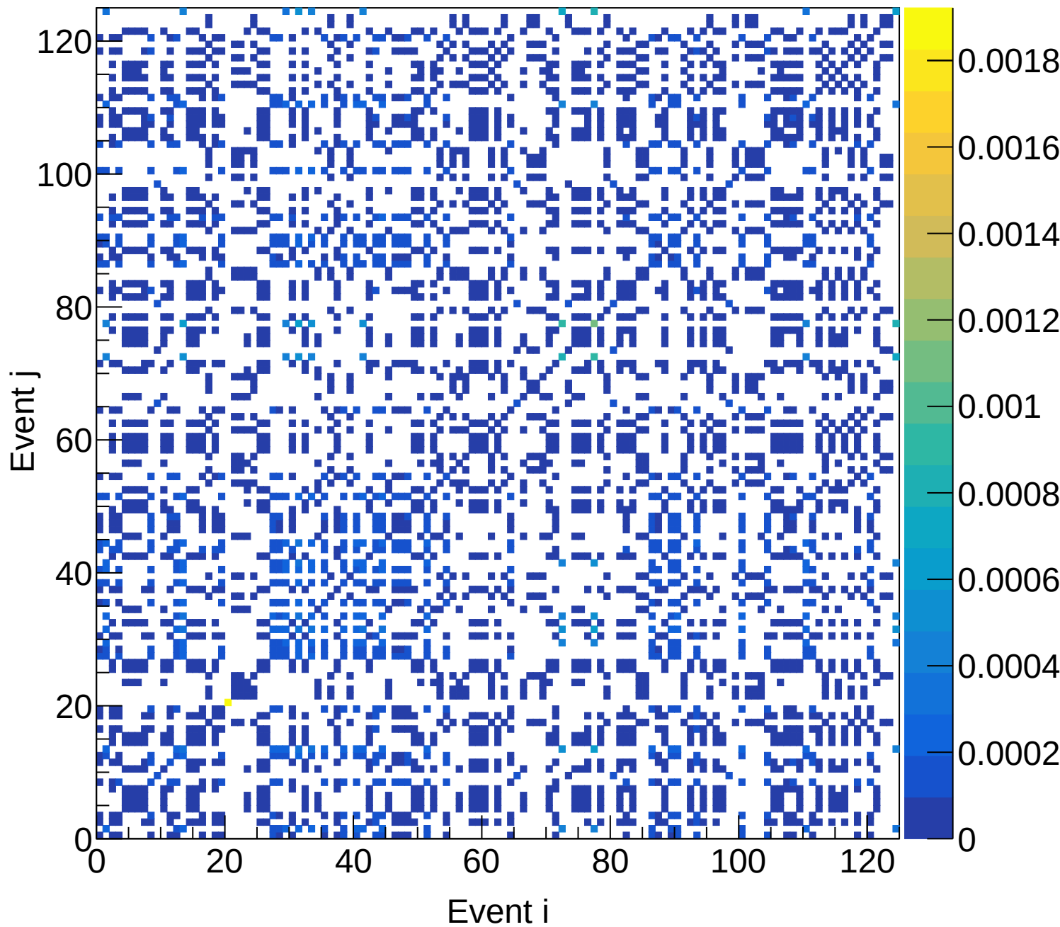
LD2 (mix) Covariance | M: [3.9, 4.2) xF: [0.35, 0.40)
