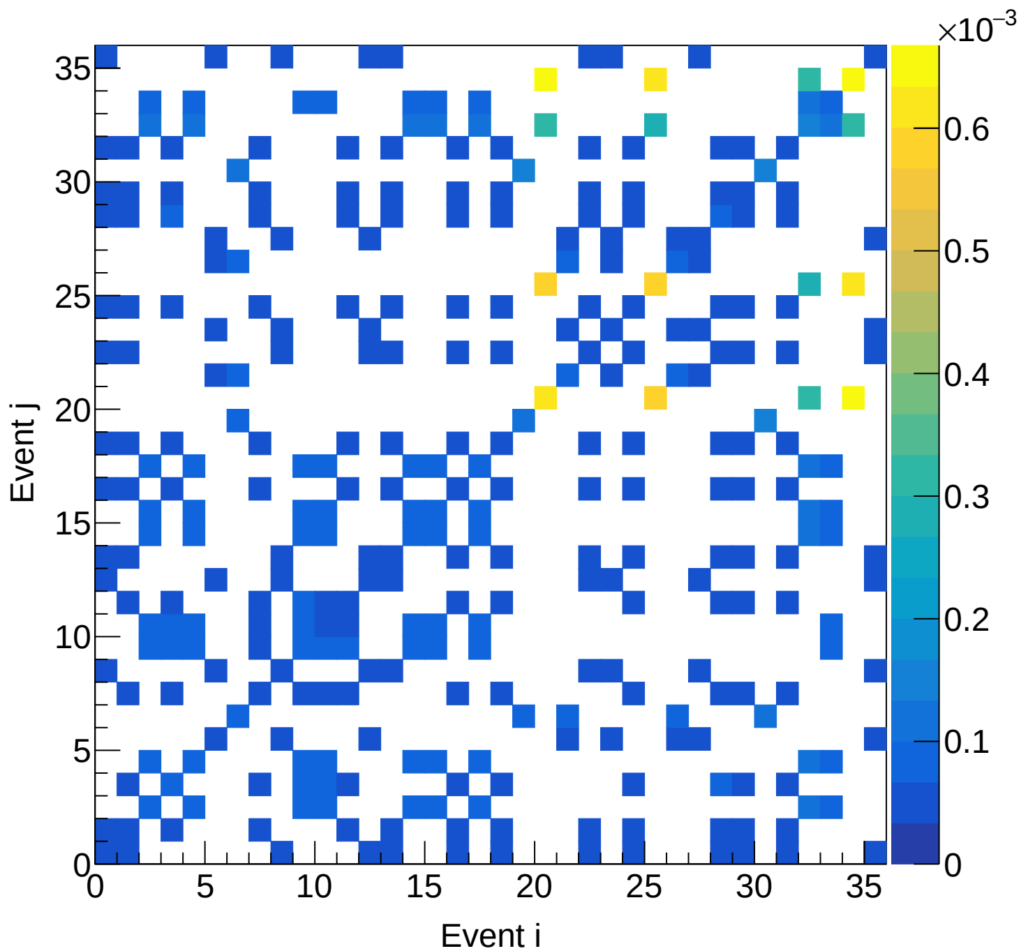
LD2 (mix) Covariance | M: [4.8, 5.1) xF: [0.35, 0.40)
