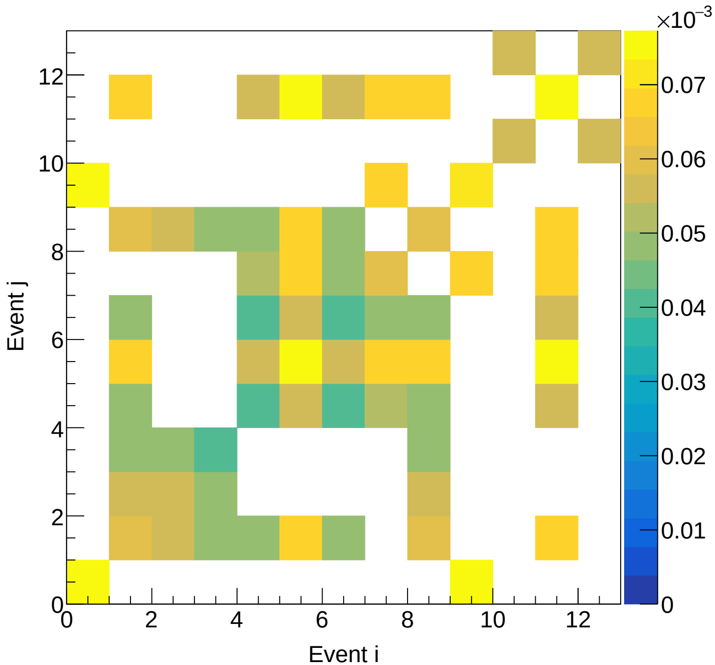
LD2 (mix) Covariance | M: [5.1, 5.4) xF: [0.35, 0.40)
