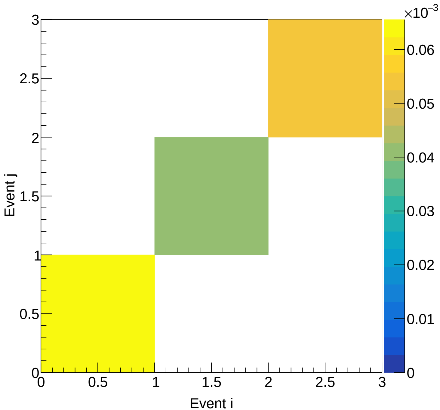
LD2 (mix) Covariance | M: [5.7, 6.0] xF: [0.35, 0.40)
