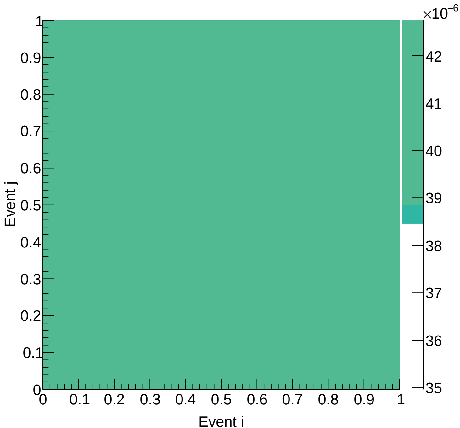
LD2 (mix) Covariance | M: [6.3, 6.6) xF: [0.35, 0.40)
