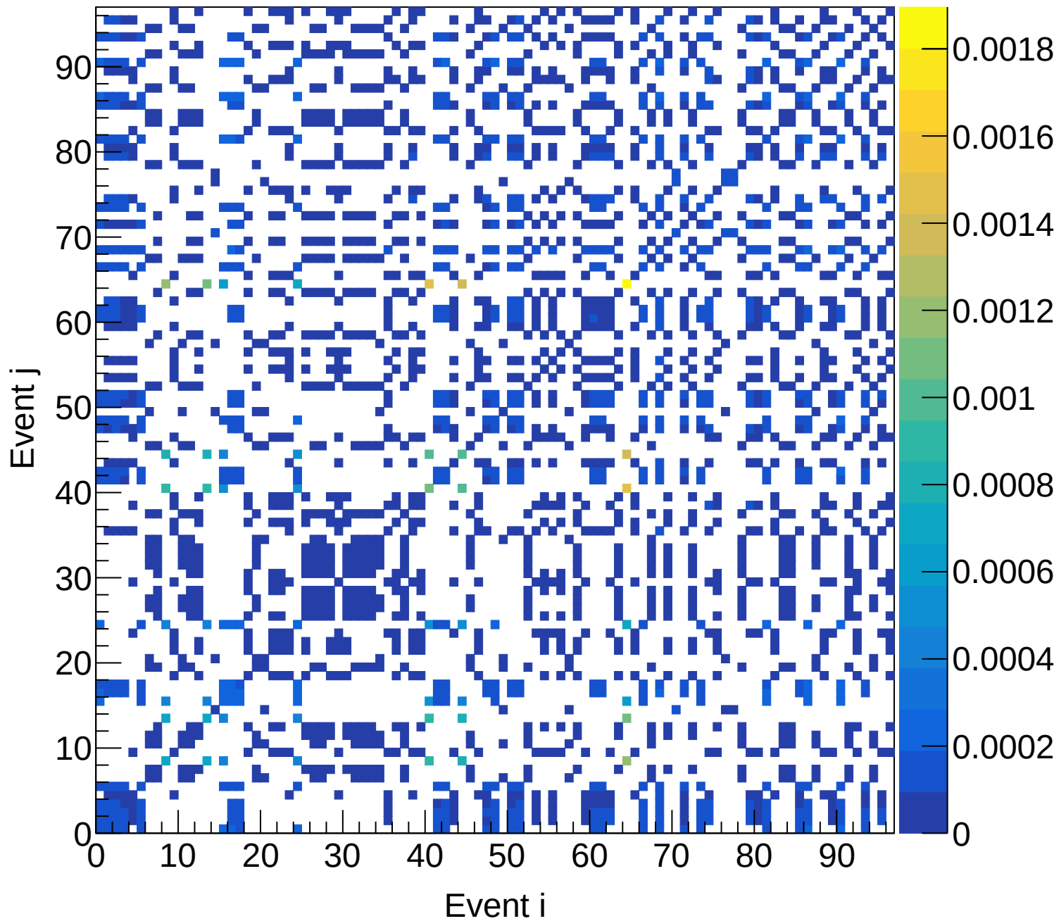
LD2 (mix) Covariance | M: [4.2, 4.5) xF: [0.40, 0.45)
