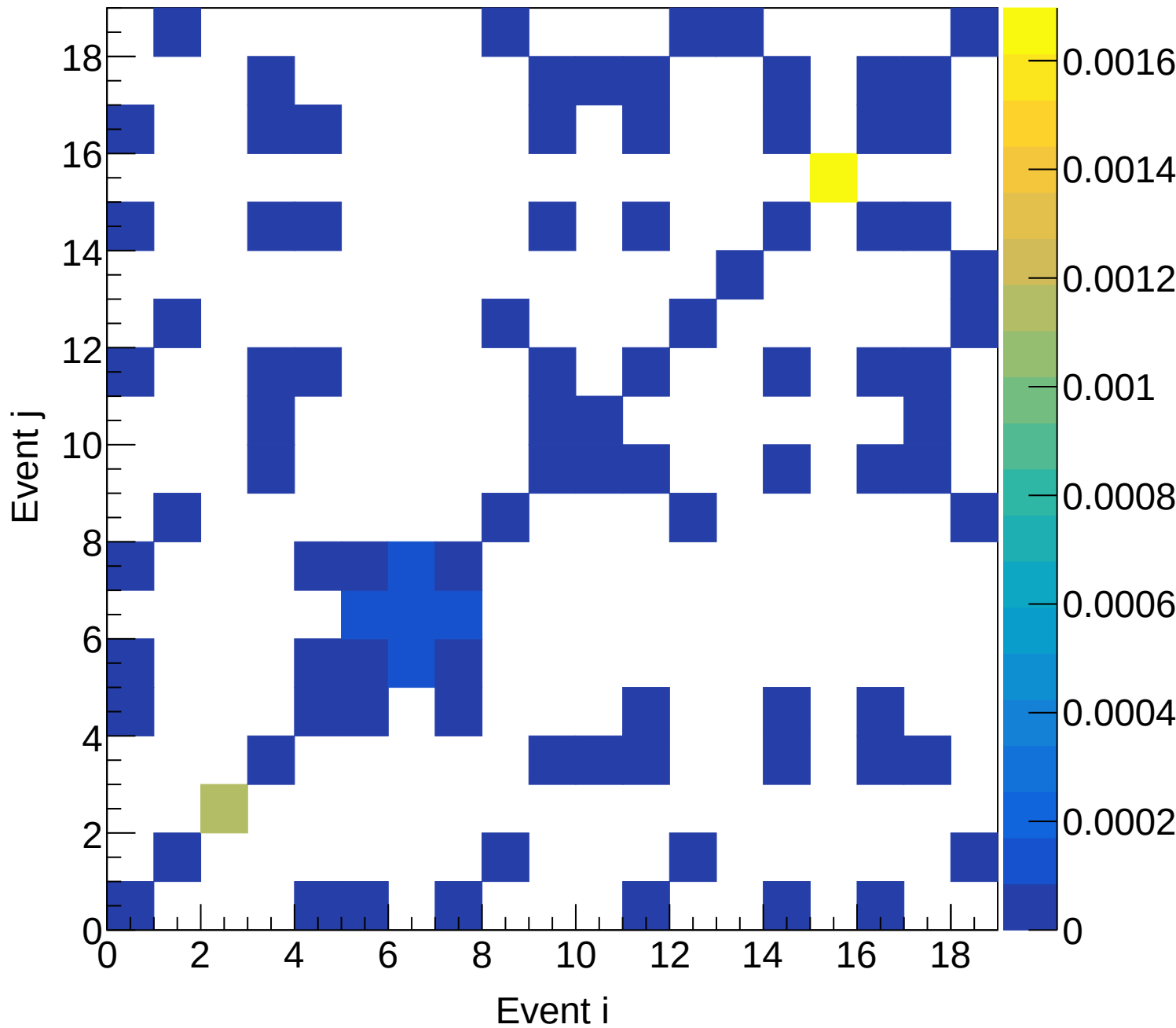
LD2 (mix) Covariance | M: [4.8, 5.1) xF: [0.40, 0.45)
