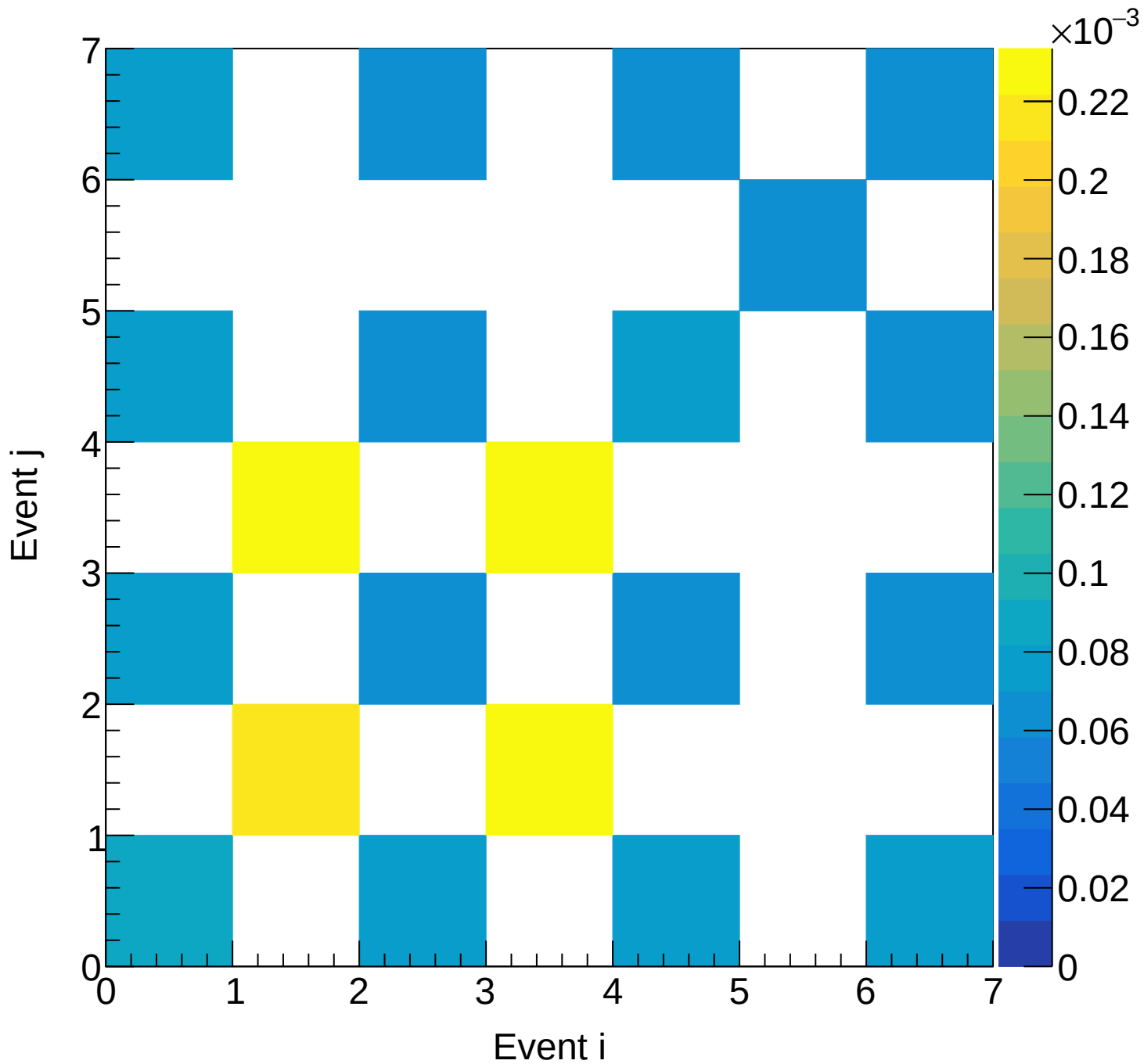
LD2 (total) Covariance | M: [4.5, 4.8) xF: [0.00, 0.05)
