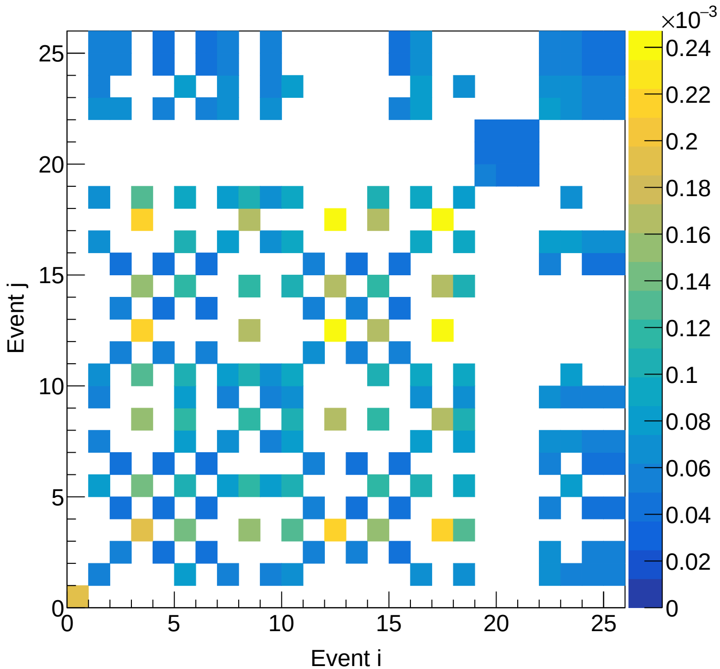
LD2 (total) Covariance | M: [5.1, 5.4) xF: [-0.05, 0.00)
