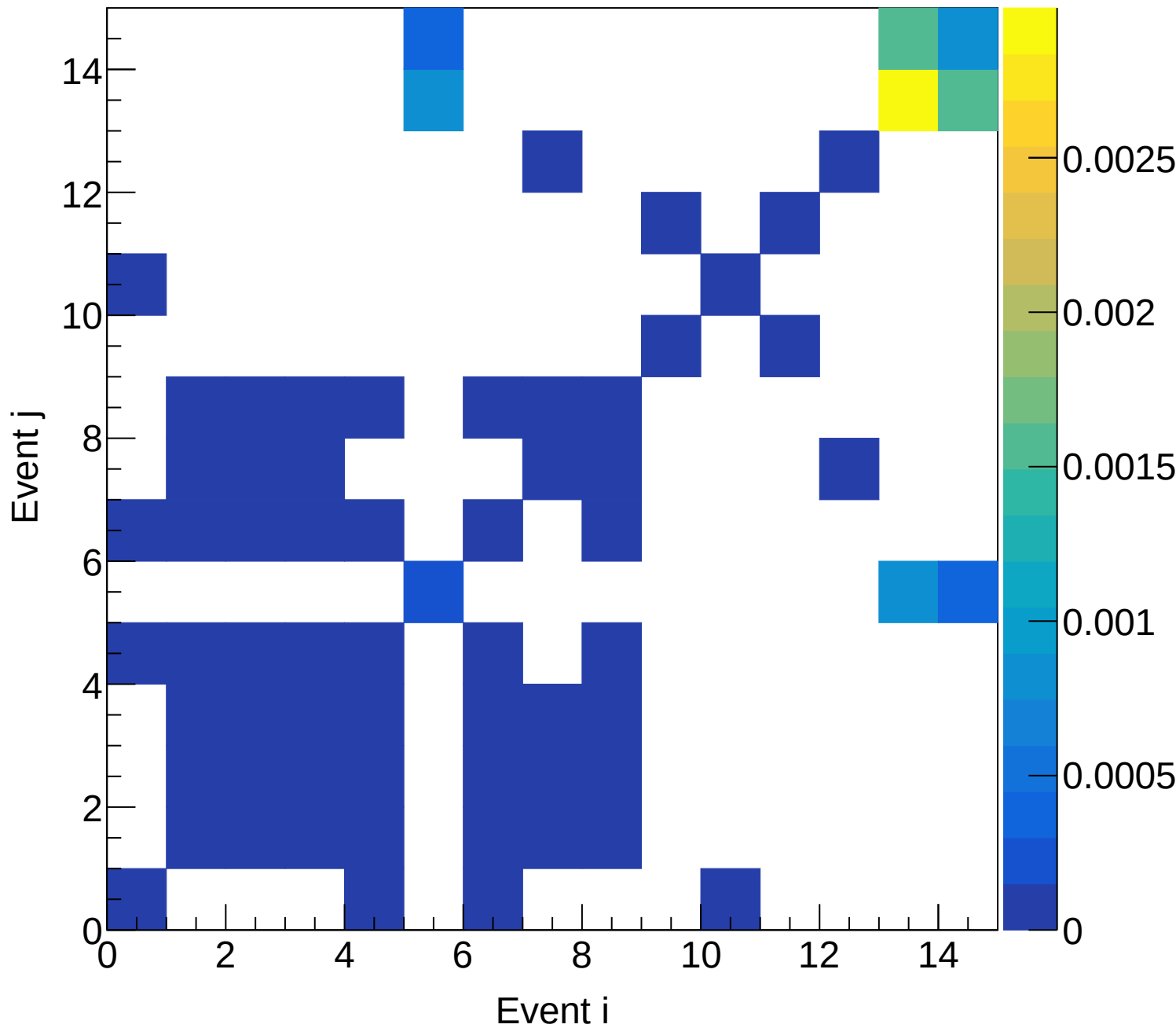
LD2 (total) Covariance | M: [6.3, 6.6) xF: [-0.05, 0.00)
