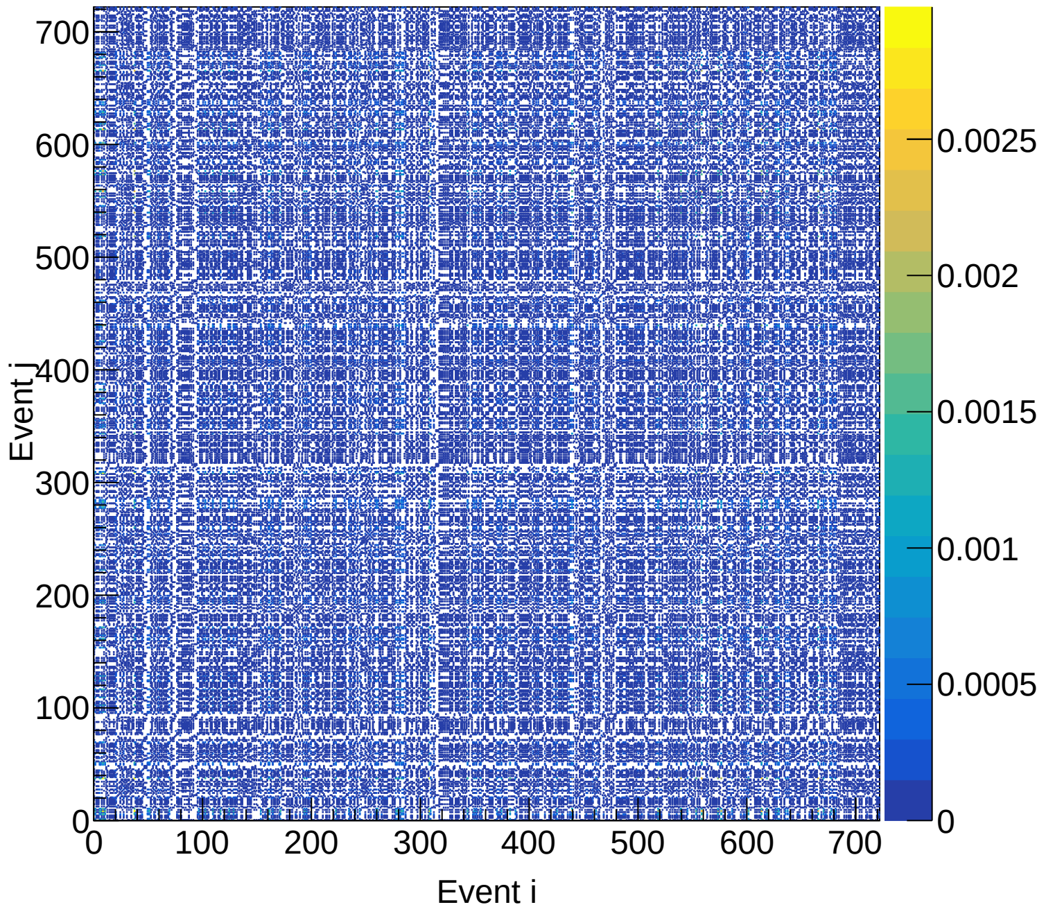
LD2 (total) Covariance | M: [4.2, 4.5) xF: [0.45, 0.50)
