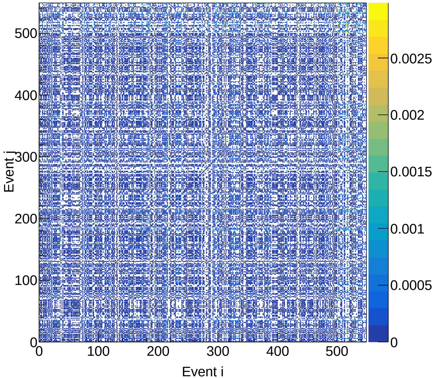
LD2 (total) Covariance | M: [4.5, 4.8) xF: [0.45, 0.50)
