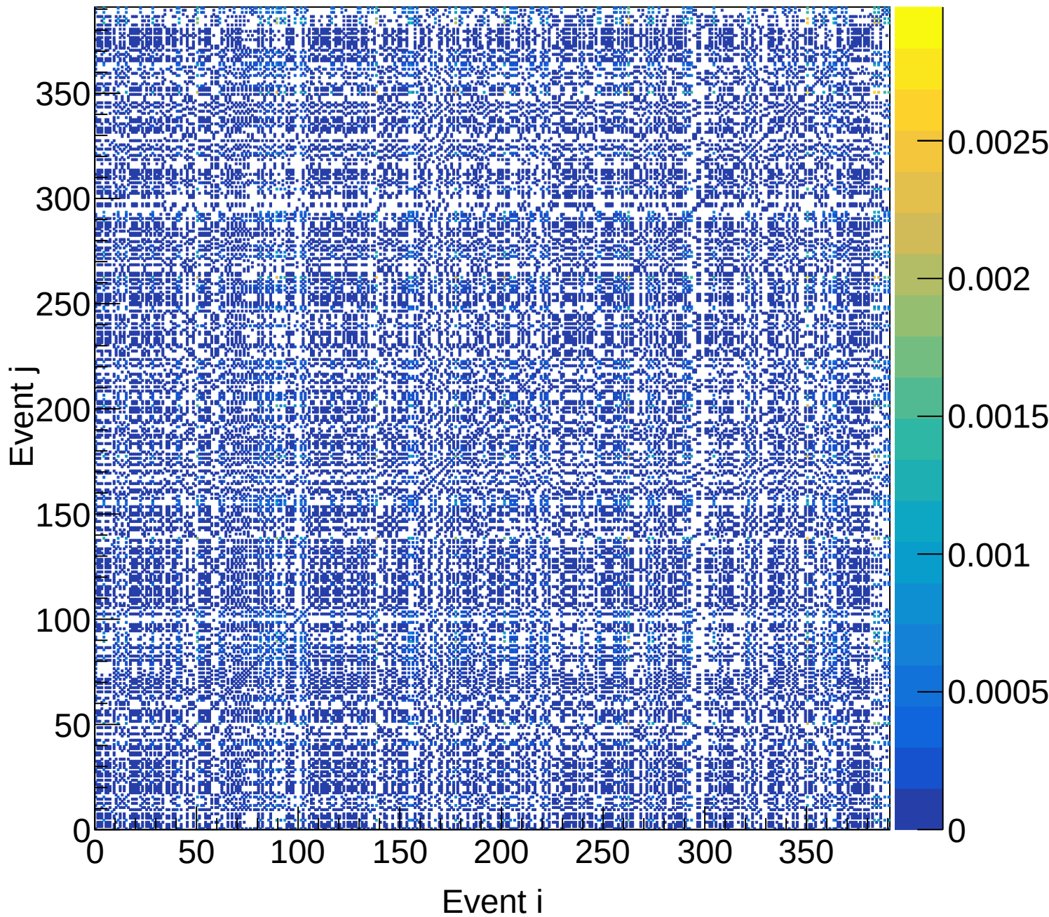
LD2 (total) Covariance | M: [4.8, 5.1) xF: [0.45, 0.50)
