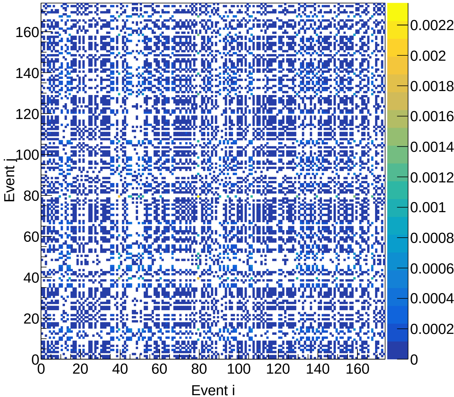
LD2 (total) Covariance | M: [5.4, 5.7) xF: [0.45, 0.50)
