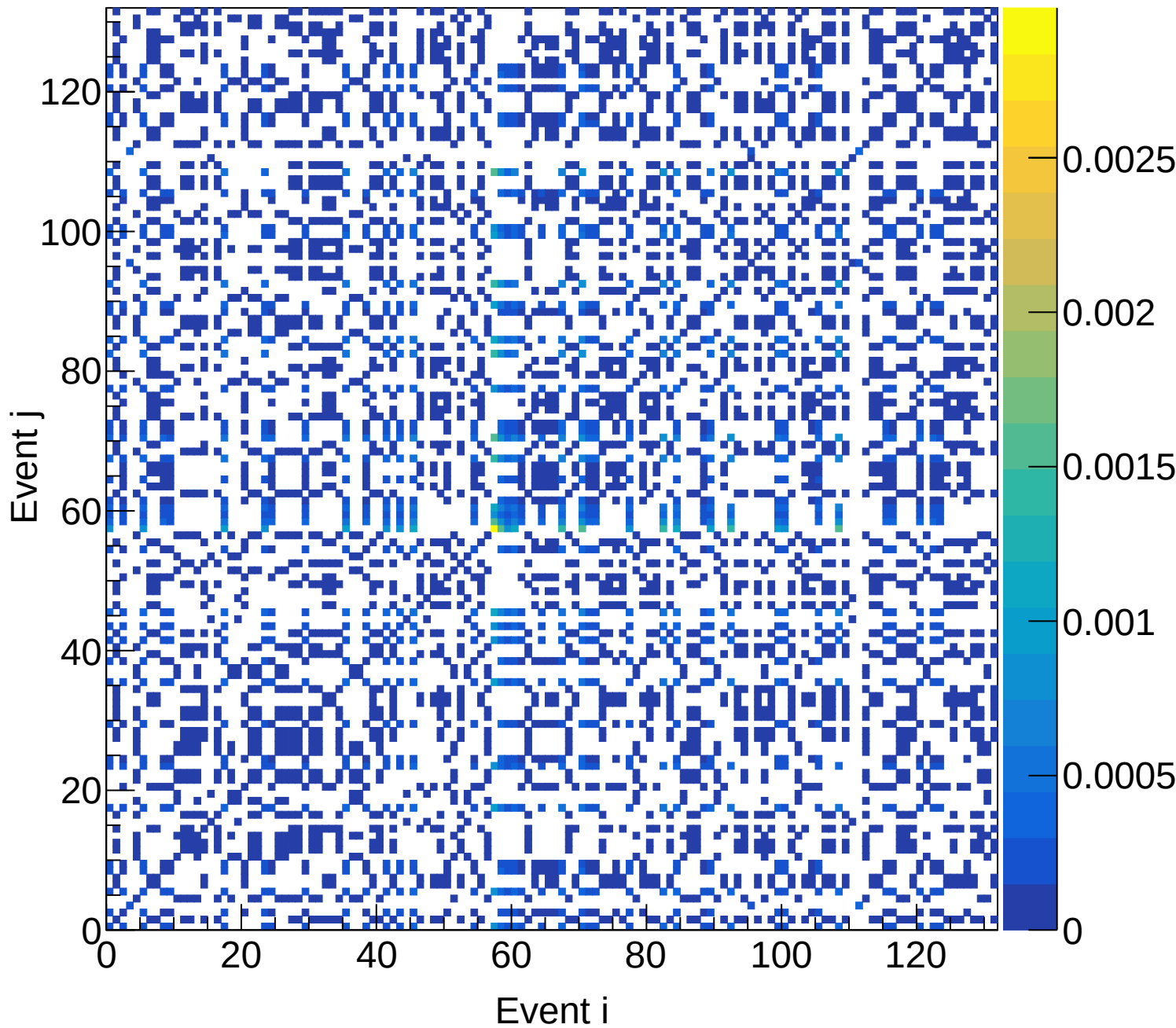
LD2 (total) Covariance | M: [5.7, 6.0) xF: [0.45, 0.50)
