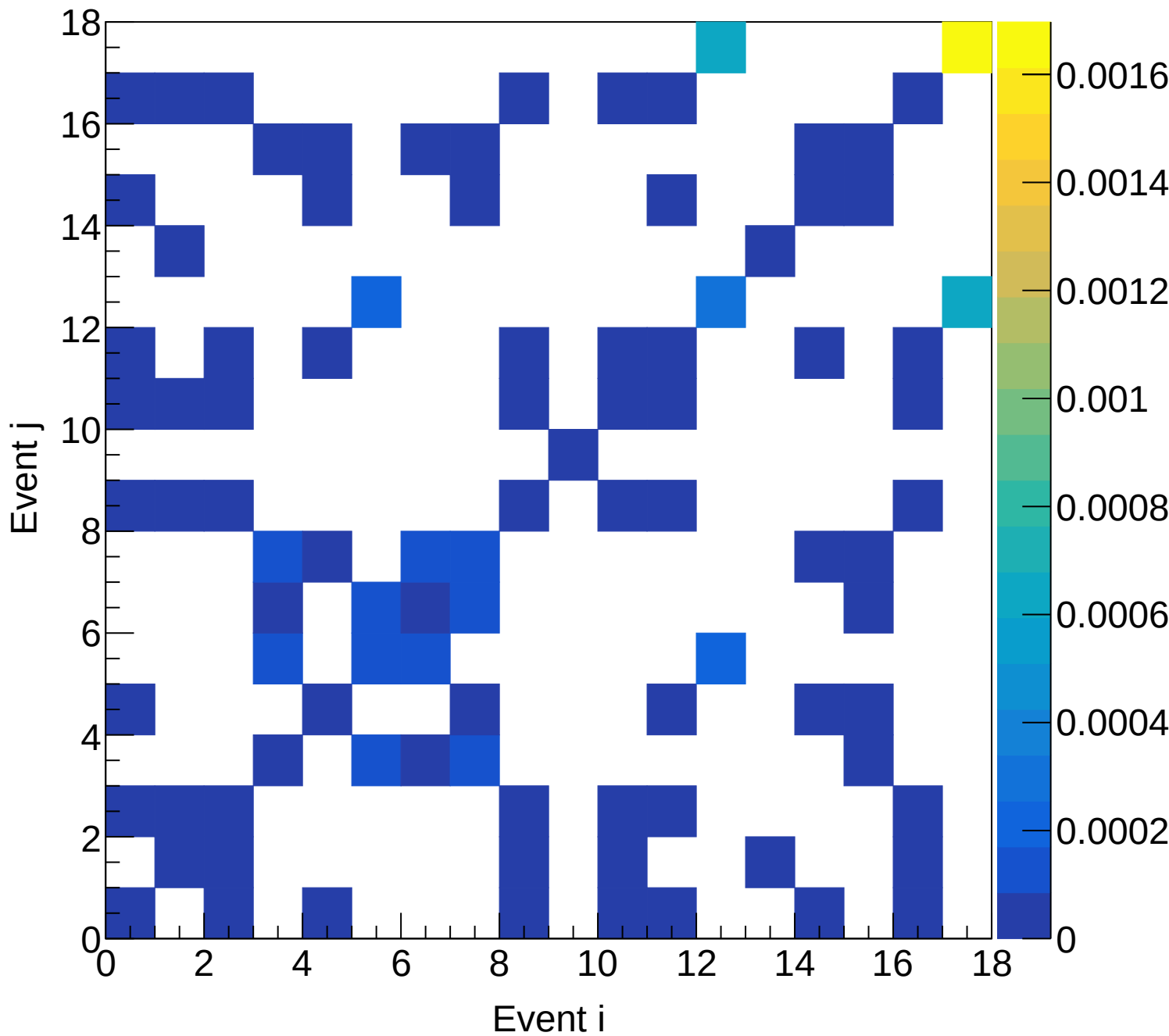
LD2 (total) Covariance | M: [6.6, 6.9) xF: [0.45, 0.50)
