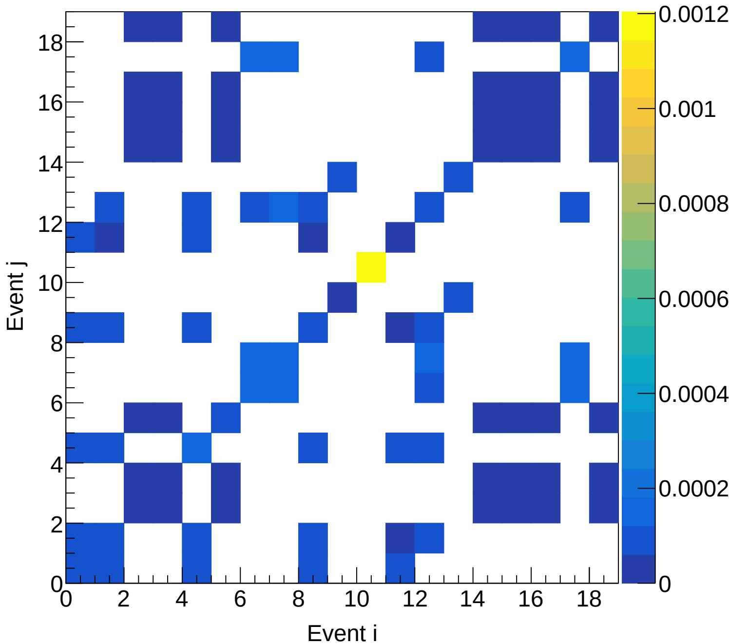
LD2 (total) Covariance | M: [6.9, 7.5) xF: [0.50, 0.55)
