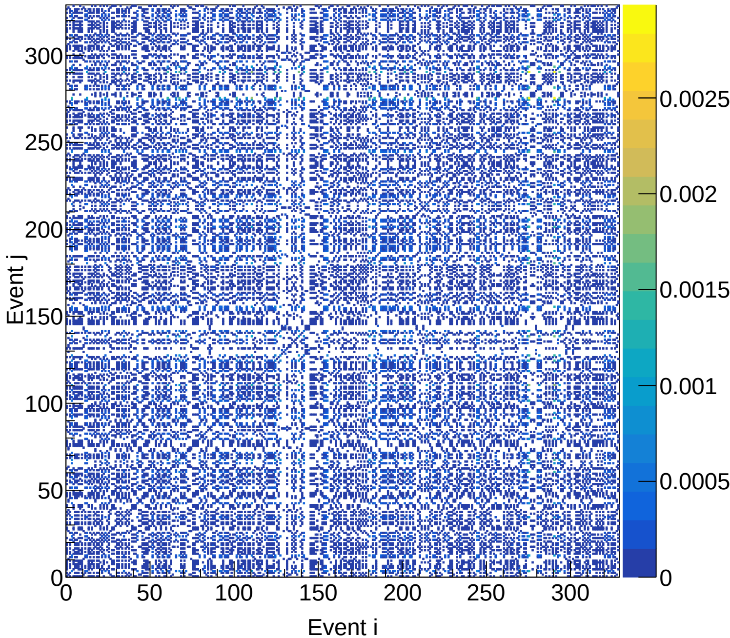
LD2 (total) Covariance | M: [4.8, 5.1) xF: [0.50, 0.55)
