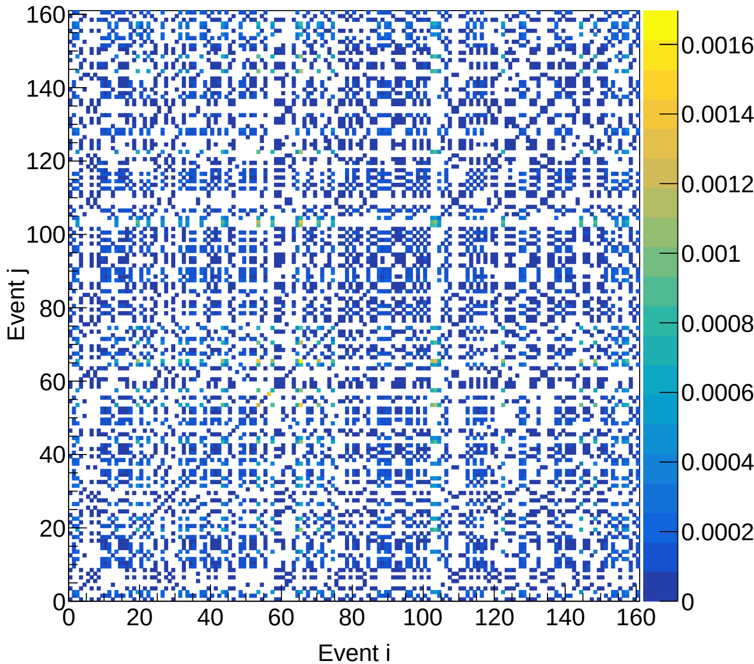
LD2 (total) Covariance | M: [5.4, 5.7) xF: [0.50, 0.55)
