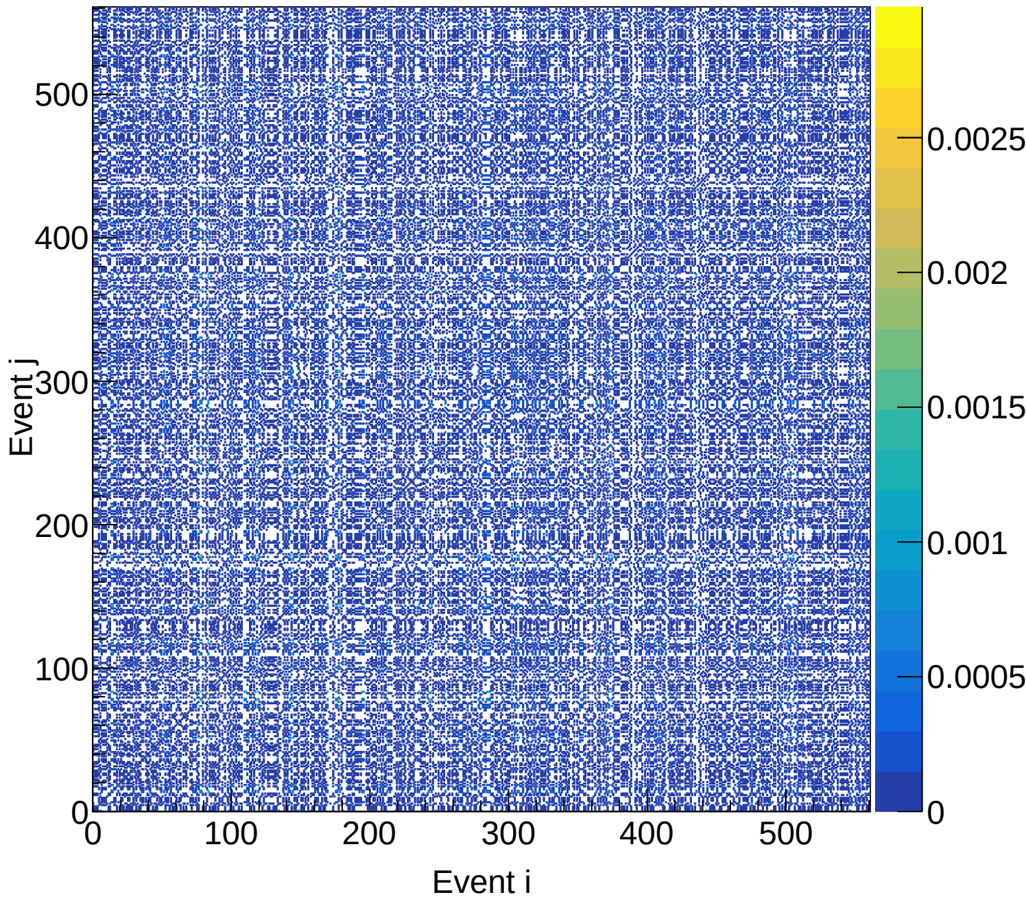
LD2 (total) Covariance | M: [4.2, 4.5) xF: [0.55, 0.60)
