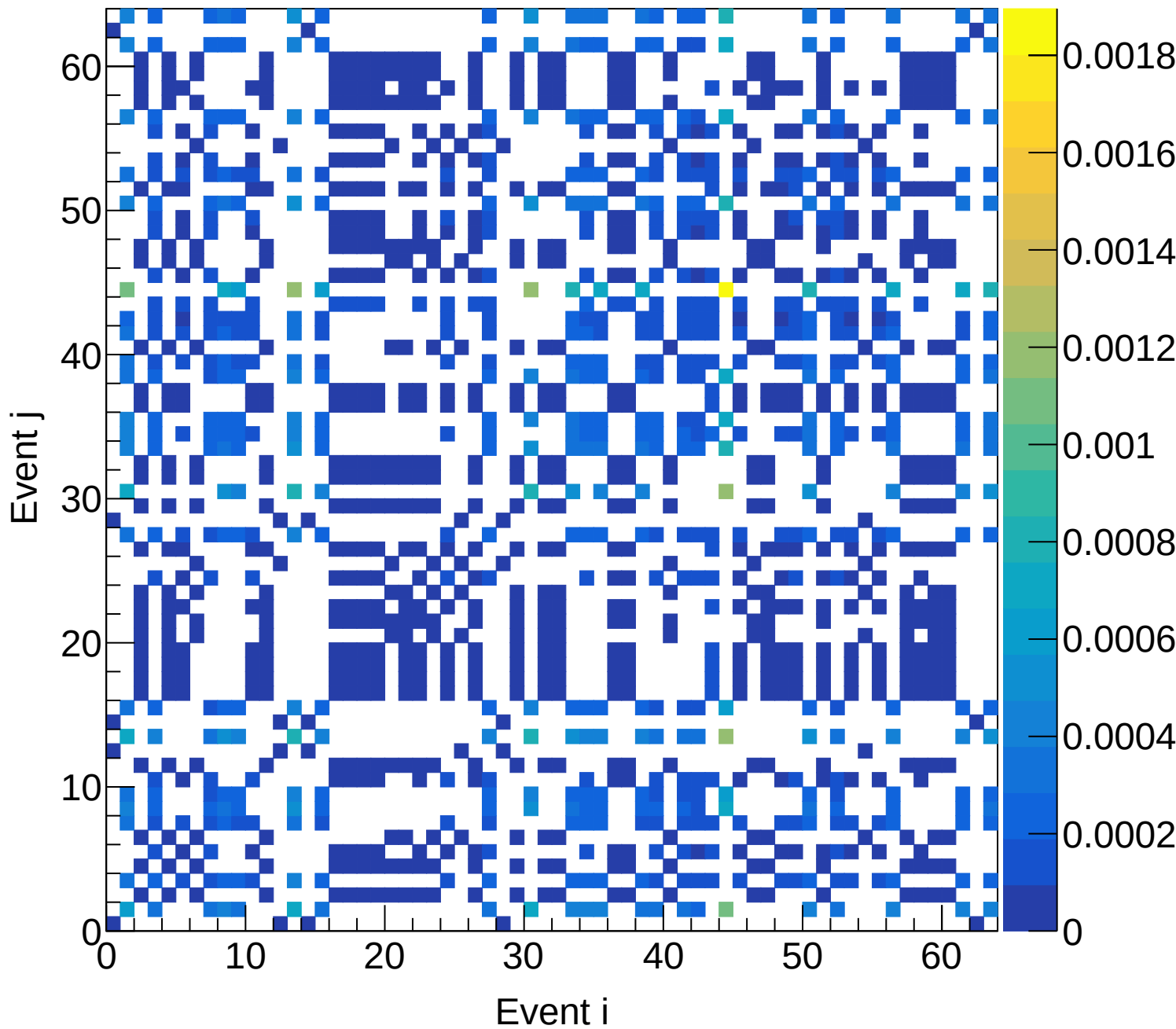
LD2 (total) Covariance | M: [5.7, 6.0) xF: [0.55, 0.60)
