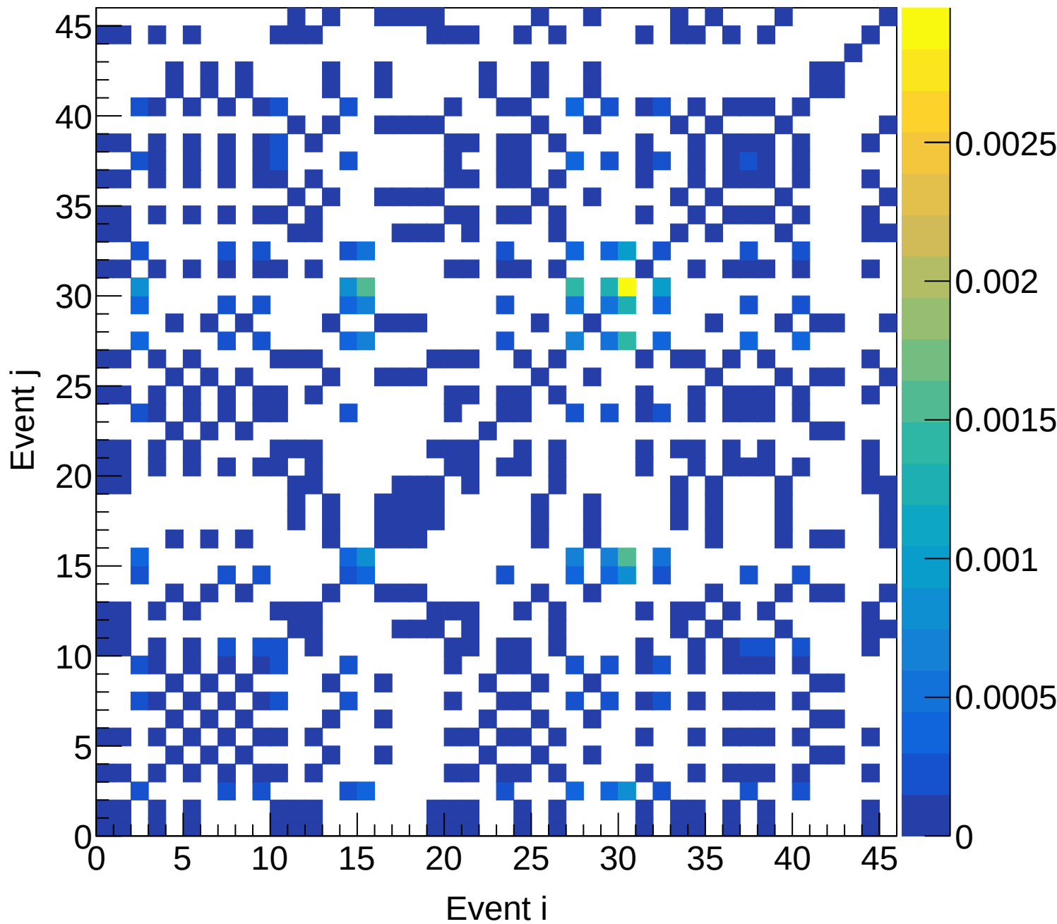
LD2 (total) Covariance | M: [6.0, 6.3) xF: [0.55, 0.60)
