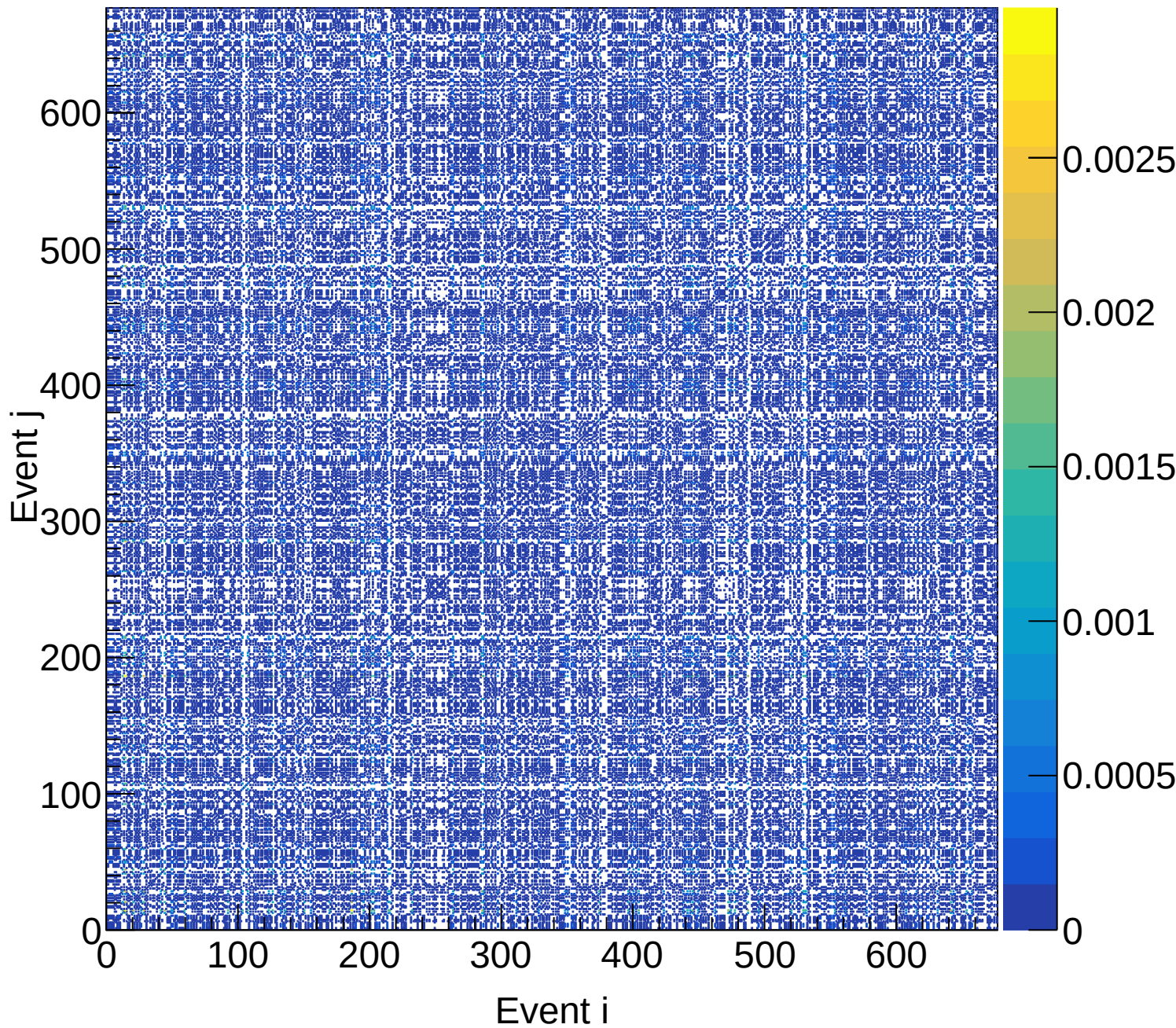
LD2 (total) Covariance | M: [3.9, 4.2) xF: [0.60, 0.65)
