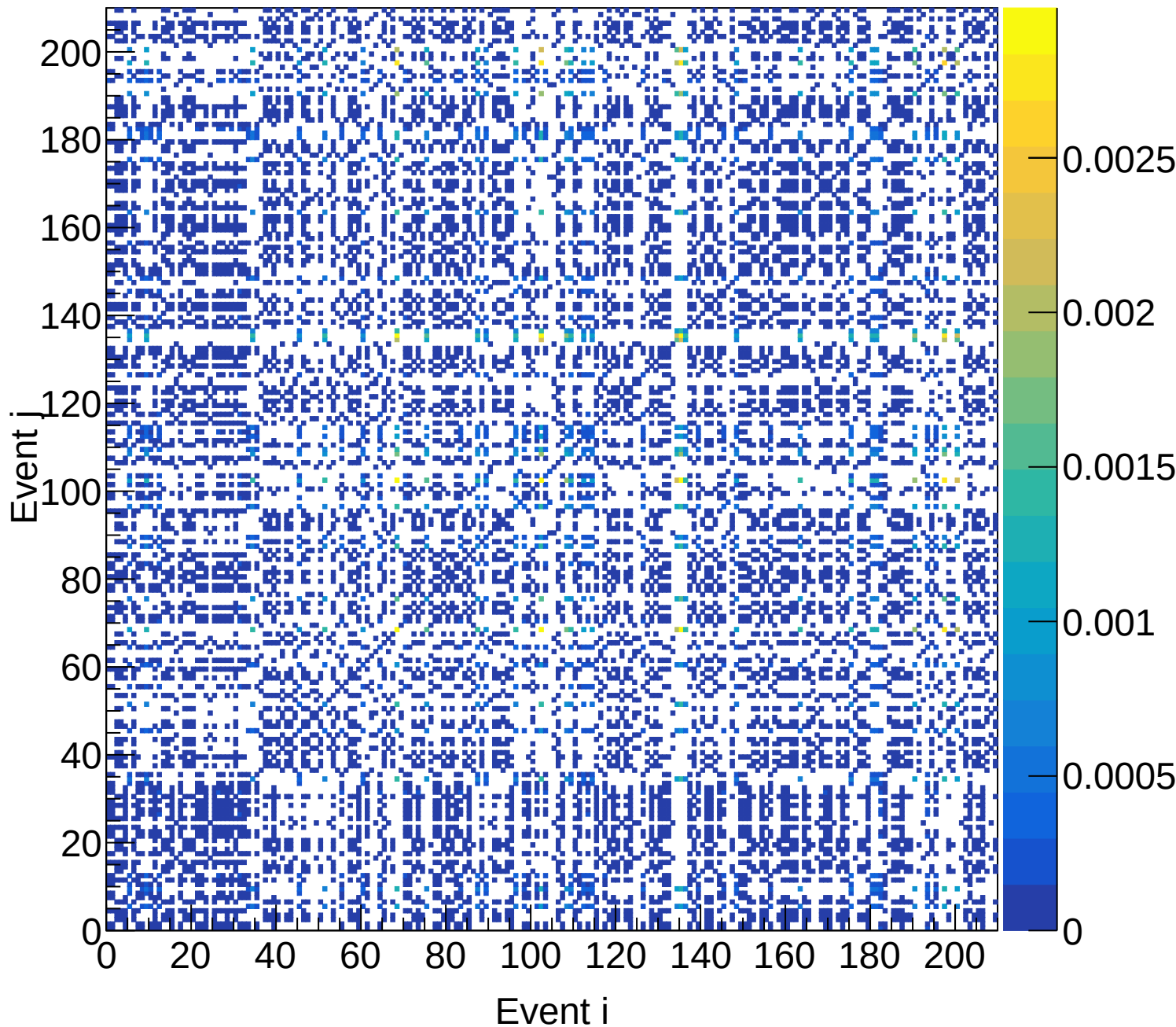
LD2 (total) Covariance | M: [4.8, 5.1) xF: [0.60, 0.65)
