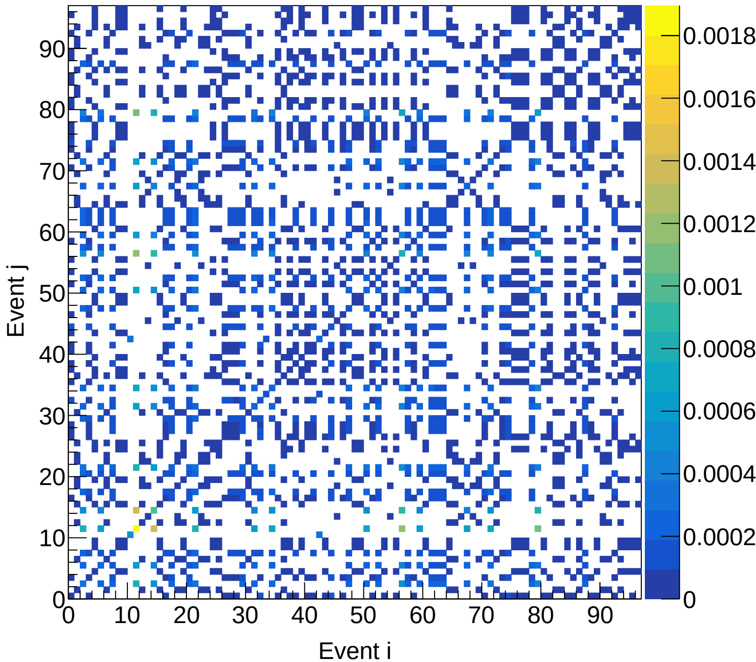
LD2 (total) Covariance | M: [5.4, 5.7) xF: [0.60, 0.65)
