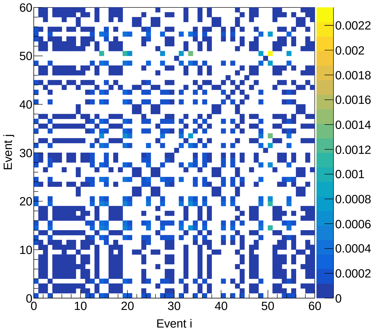
LD2 (total) Covariance | M: [5.7, 6.0] xF: [0.60, 0.65]
