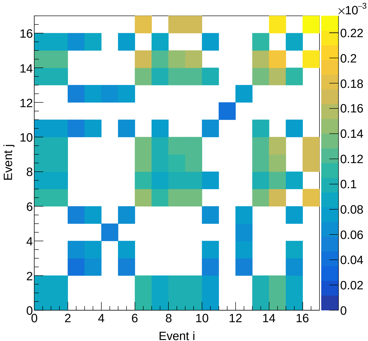
LD2 (total) Covariance | M: [6.6, 6.9) xF: [0.60, 0.65)
