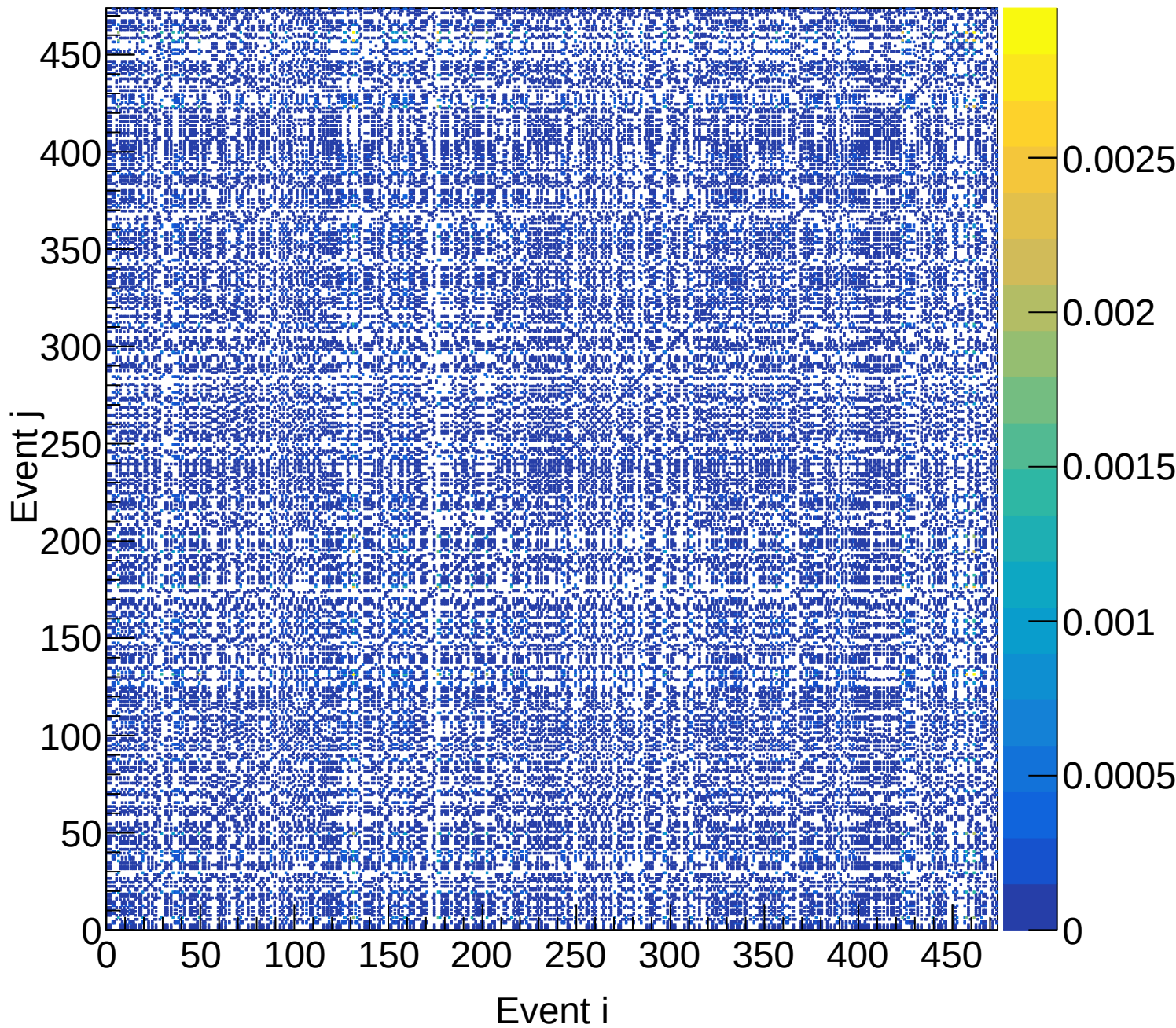
LD2 (total) Covariance | M: [3.9, 4.2) xF: [0.65, 0.70)
