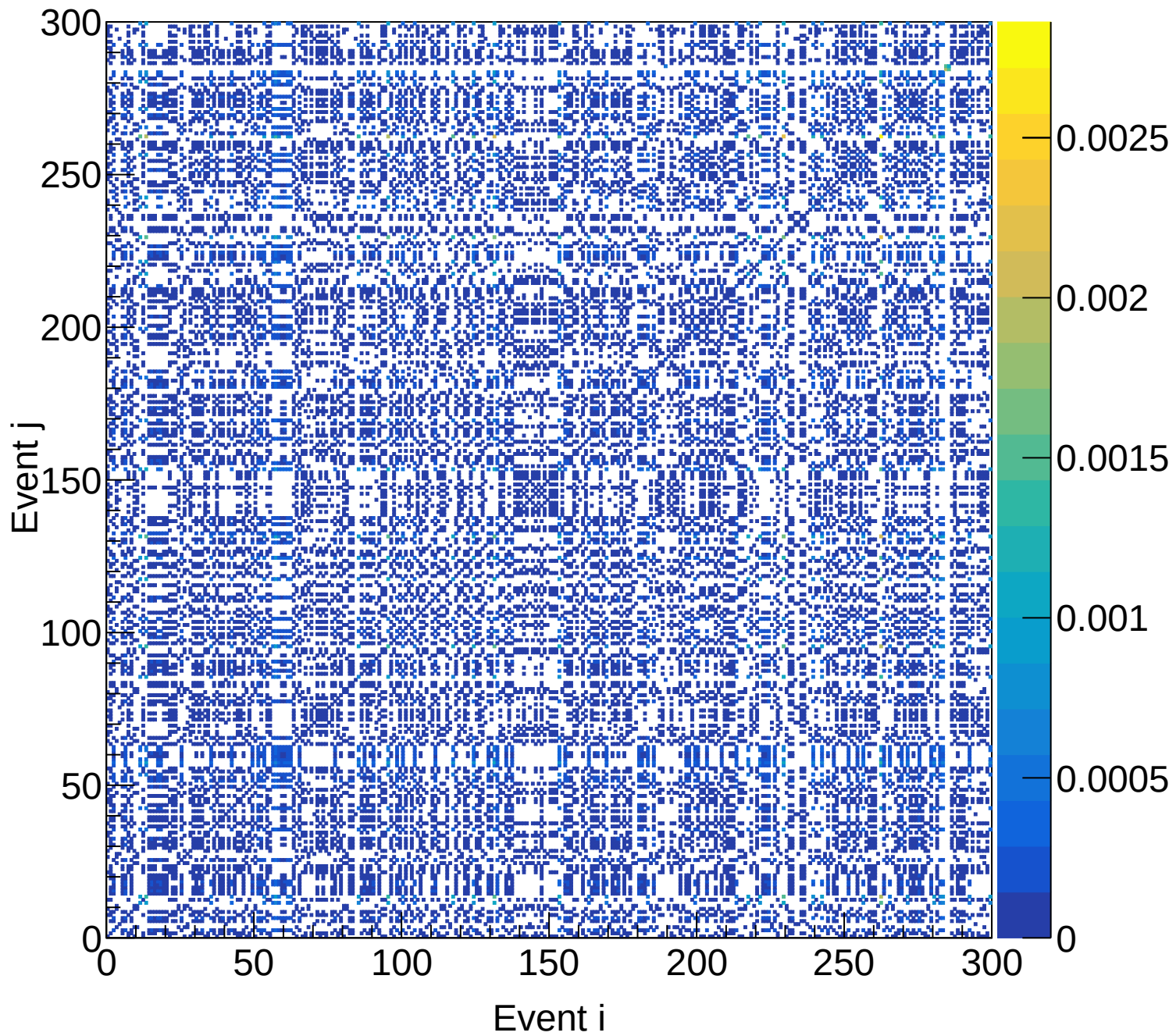
LD2 (total) Covariance | M: [4.2, 4.5) xF: [0.65, 0.70)
