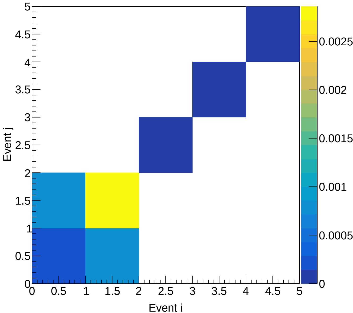
LD2 (total) Covariance | M: [6.9, 7.5) xF: [0.65, 0.70)
