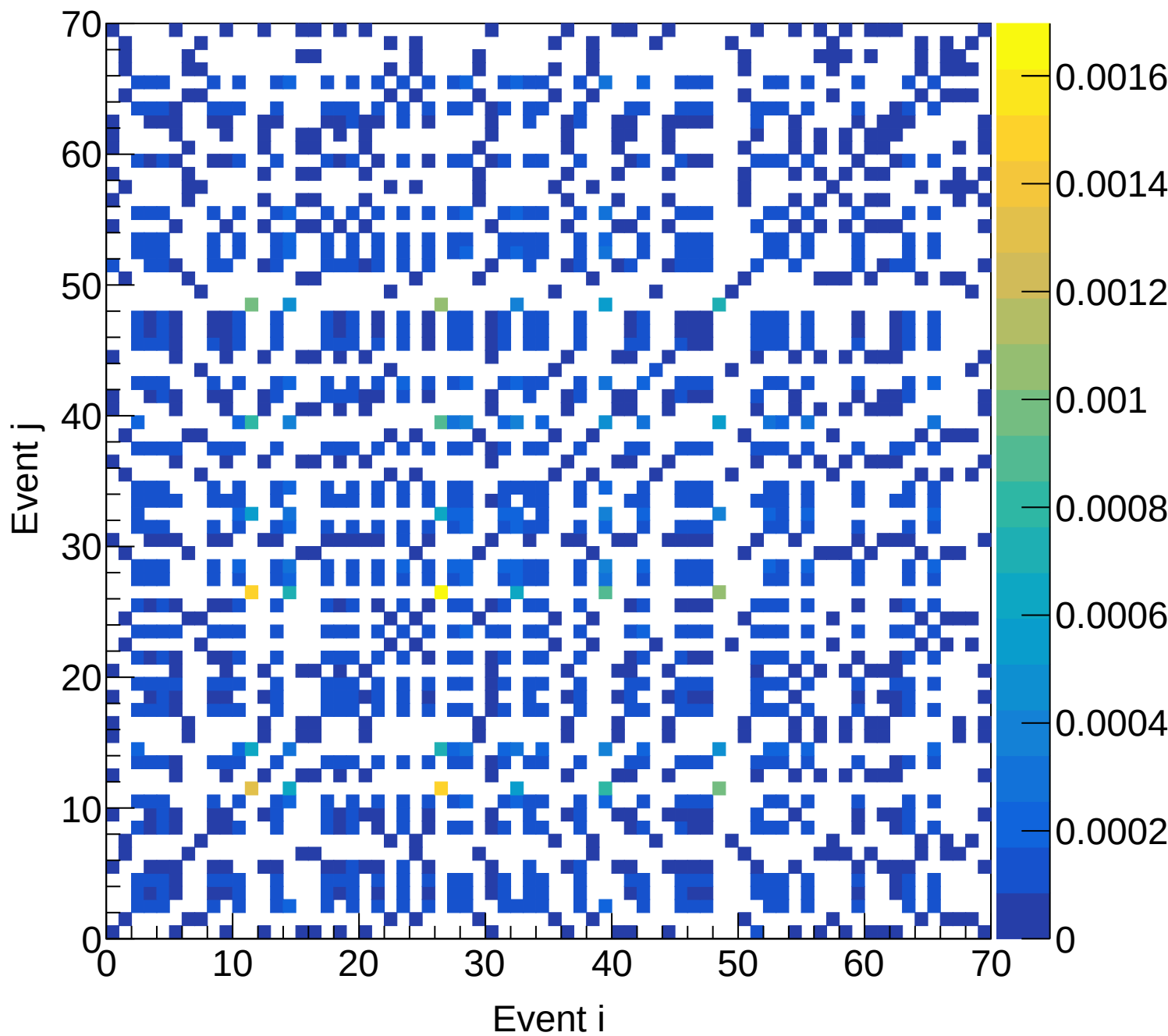
LD2 (total) Covariance | M: [5.1, 5.4) xF: [0.65, 0.70)
