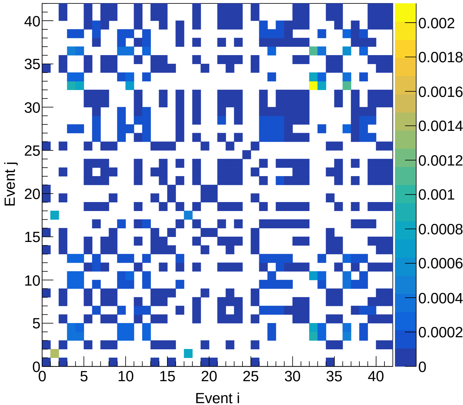
LD2 (total) Covariance | M: [5.7, 6.0] xF: [0.65, 0.70)
