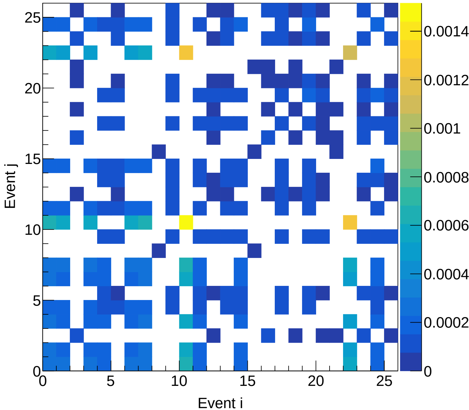
LD2 (total) Covariance | M: [6.0, 6.3) xF: [0.65, 0.70)
